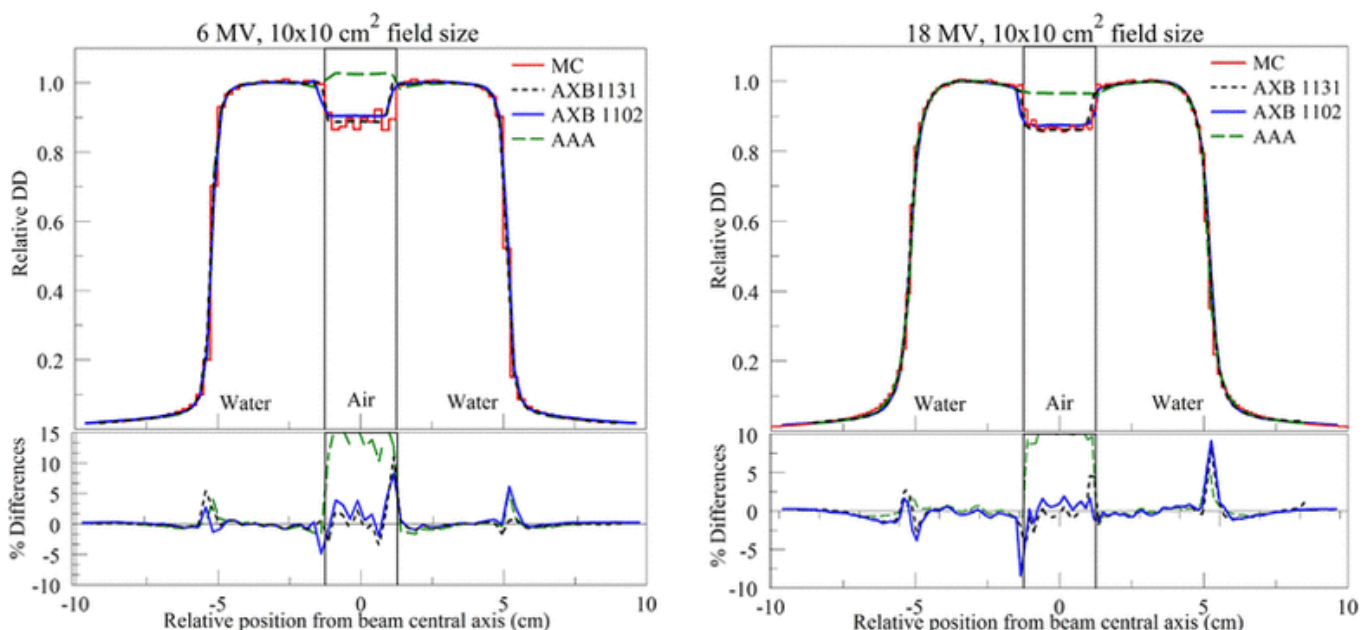
Fig. 5 Lateral profiles through the center of the rectangular air cavity for 6 MV (left) and 18 MV (right) beams.
