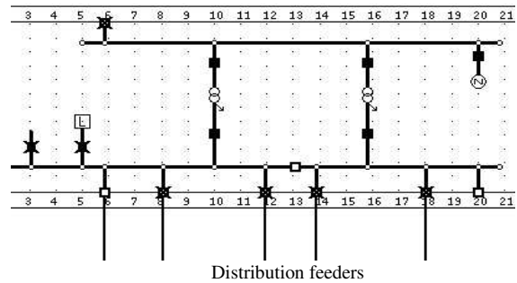
Figure 1: Smithton substation's one-line diagram
