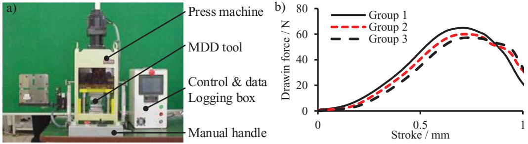
Figure 3. (a) Micro deep drawing machine and (b) drawing forces of each material group.
