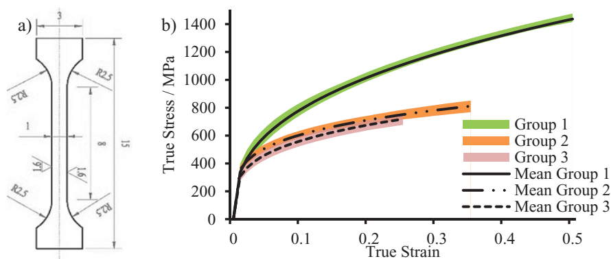
Figure 2. (a) Tensile sample and (b) true strain stress curve of each material group.
