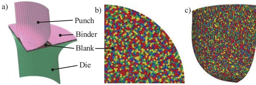
Figure 4. (a) MDD simulation model, (b) voronoi blank model and (c) drawn cup.
