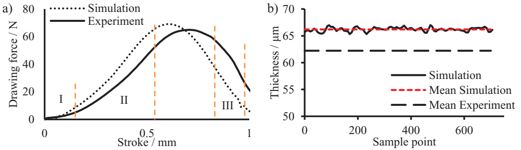
Figure 5. (a) Drawing force and (b) thickness distribution.
