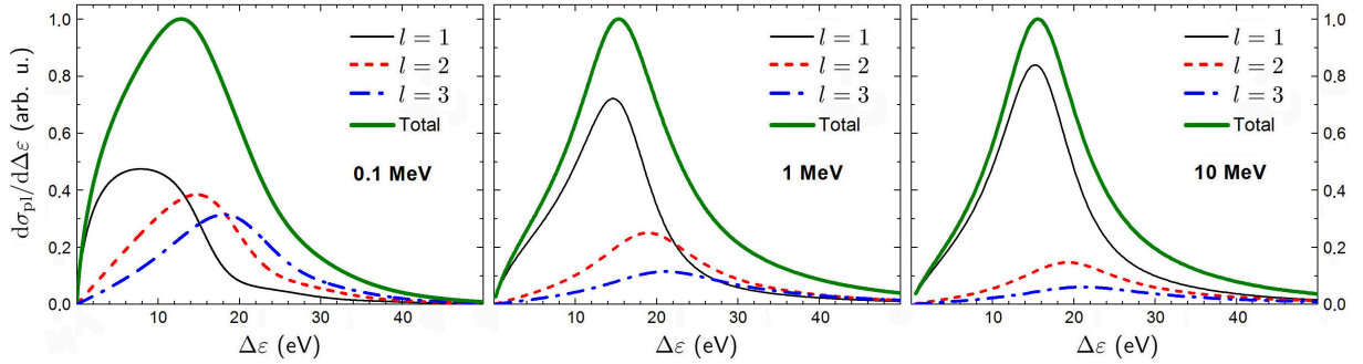
FIG. 2. Relative contribution of different multipole terms to the single differential cross section d\sigma_{pl}/d\Delta\varepsilon of C_{60} fullerene irradiated by 0.1, 1, 10 MeV protons as a function of the energy loss.
