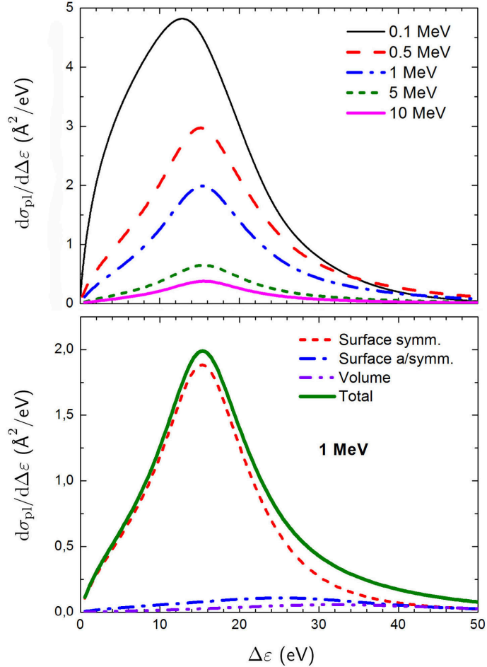
FIG. 1. Upper panel: contribution d\sigma_{\text{pl}}/d\Delta\varepsilon of the plasmon excitations to the single differential cross section of \text{C}_{60} fullerene irradiated by fast protons of different incident energies as a function of the energy loss. Lower panel illustrates the contribution of different plasmon excitations to the cross section d\sigma_{\text{pl}}/d\Delta\varepsilon of \text{C}_{60} irradiated by a 1 MeV proton.
