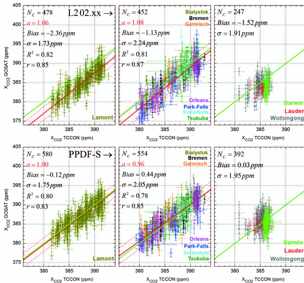
Fig. 6. Correlation diagrams between GOSAT and ground-based TCCON measurements of X_{\text{CO}_2} for two GOSAT retrieval algorithms, PPDF-S (bottom panels) and NIES L2 02.xx (top panels), and for three sets of TCCON sites, over Lamont (left-hand panels), over the other seven Northern Hemisphere sites (middle panels), and over three Southern Hemisphere sites (right-hand panels). The GOSAT single scans were selected during 14 months from June 2009 within a 5^\circ radius latitude/longitude circle centered over each TCCON station. The analyzed ground-based FTS data were mean values measured within \pm 1 h of the GOSAT overpass time. Red lines correspond to the best fits, and the green line represents one-to-one correspondence. The number of coincident soundings and characteristics of statistical relationships between ground-based FTS and GOSAT X_{\text{CO}_2} for each set of TCCON stations is listed in the legend of each panel.
