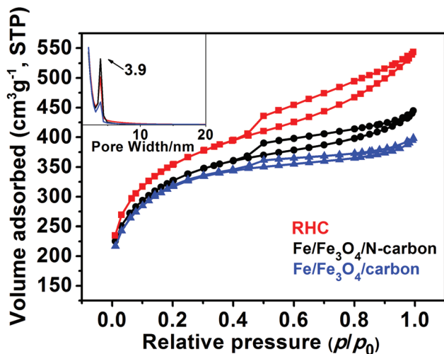
Fig. 4 N_2 adsorption isotherms of RHC, Fe/Fe_3O_4/N -carbon and Fe/Fe_3O_4/carbon .
