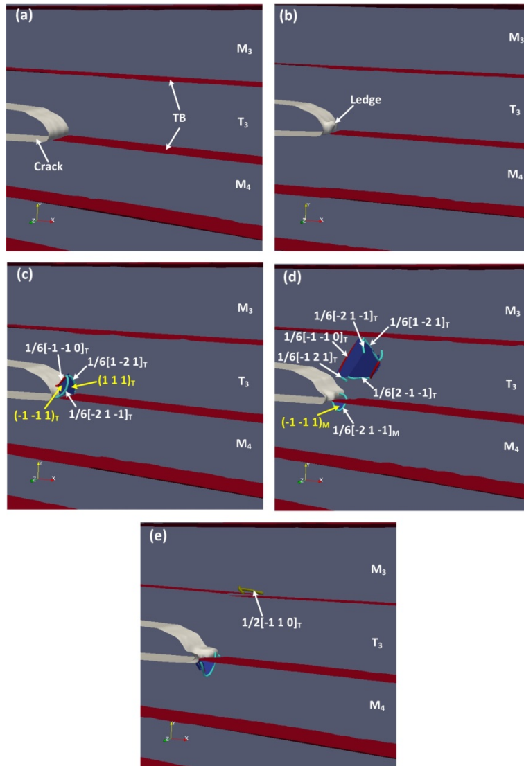
Fig. 9 Dislocation activities around the crack tip for the 40 K case: (a) \varepsilon = 2.52\% ; (b) \varepsilon = 2.537\% ; (c) \varepsilon = 2.559\% ; (d) \varepsilon = 2.59\% ; (e) \varepsilon = 2.604\% .
