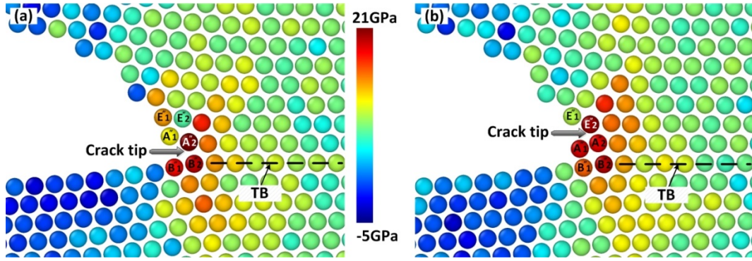
Fig. 13 Stress along the Y direction ( \sigma_y ) for the 40 K case at \varepsilon = 2.529\% : (a) 11.3 \text{ \AA} \leq Z \leq 13 \text{ \AA} ; (b) 17.7 \text{ \AA} \leq Z \leq 19.3 \text{ \AA} .
