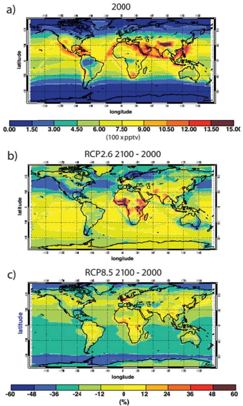
Fig. 7 (a) Annual average surface \bullet\text{OH} concentration, mean of 14 models, for the year 2000. (b) Model-mean % change in surface \bullet\text{OH} concentrations in 2100 relative to 2000, for the IPCC RCP 2.6 emission scenario; (c) same for RCP 8.5 scenarios (From Voulgarakis et al. 144 ).
