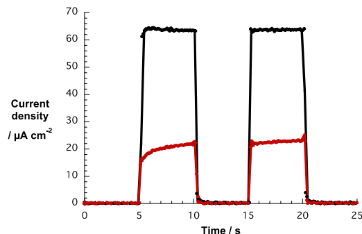
Fig. 10 Photocurrent responses versus time of DSSCs based on TiO 2 -T (red) and TiO 2 -S (black) electrodes soaked with G7a in THF for 120 hours.
