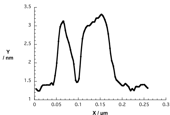
Fig. 4 Upper part – AFM image of a spin-coated dispersion of G7b in THF onto silicon oxide wafer. Lower part – Corresponding height profile across line 1. Height profiles across lines 2, 3, and 4 are shown in Figure S5.
