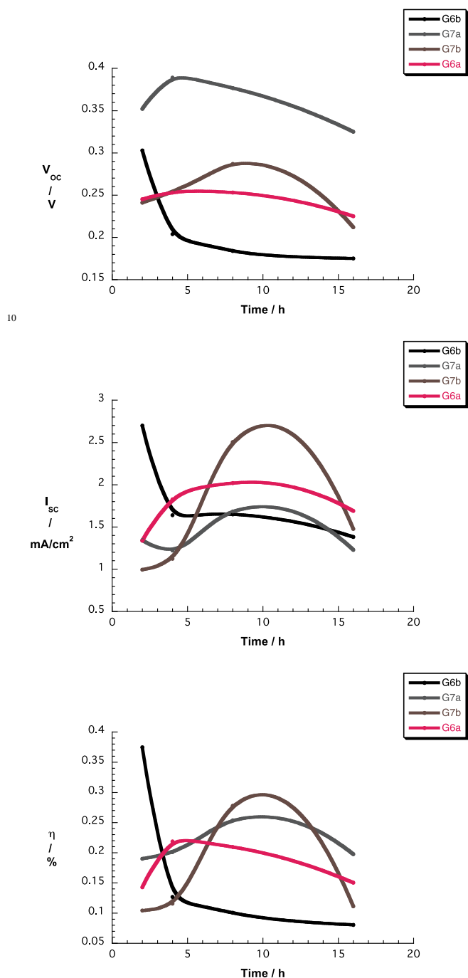
Fig. 11 Upper part – V_{oc} as a function of soaking time for devices using nanographene / porphyrin hybrids in THF. Central part – I_{sc} as a function of soaking time for devices using nanographene / porphyrin hybrids in THF. Lower part – \eta as a function of soaking time for devices using nanographene / porphyrin hybrids in THF
