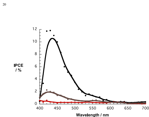
Fig. 12 IPCE spectra for DSSCs with G6b (black spectrum), graphene (red spectrum), and 6b (brown spectrum).
