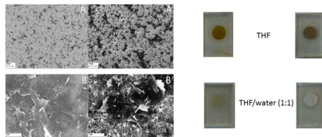
Fig. 8 Left – SEM images of TiO 2 -T (left) and TiO 2 -S (right) soaked with G7a THF for 120 hours at low (A) and high (B) magnification, respectively. Right – Photographs of TiO 2 -T (left) and TiO 2 -S (right) soaked with G7a in THF and THF/water (1:1 v/v) for 120 hours.
