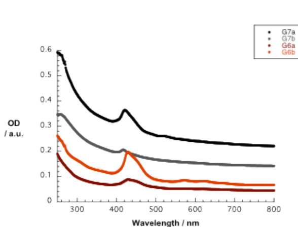
Fig. 6 Absorption spectra of G6a/b and G7a/b in THF. The initial concentration of 6a/b and 7a/b was 2 \times 10^{-5} M. The amount of dispersed graphene was calculated using the absorption coefficient a = 36.0 mL / mg cm at 660 nm. 52
