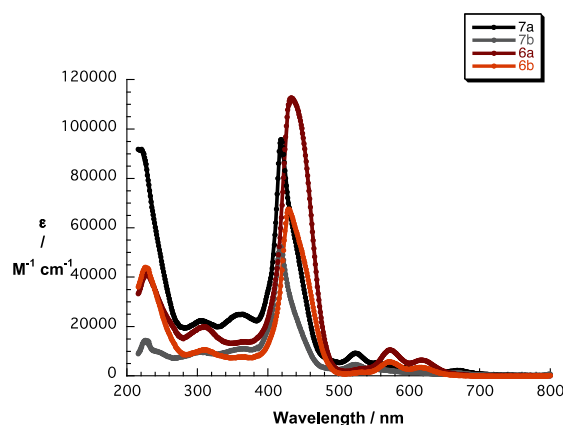
Fig. 1 Absorption spectra of 6a/b and 7a/b in THF.
