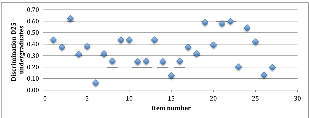
Figure 7: item discrimination D 25 for undergraduates
