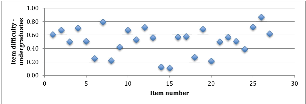
Figure 5: item difficulty for undergraduates
