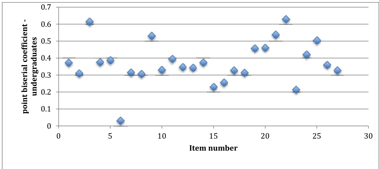
Figure 8: point biserial coefficient for undergraduates
