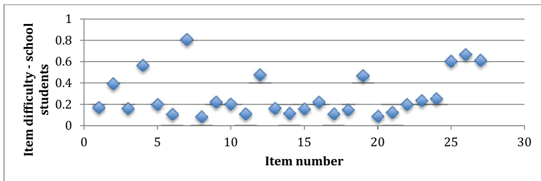
Figure 1: Item difficulty for high school students
