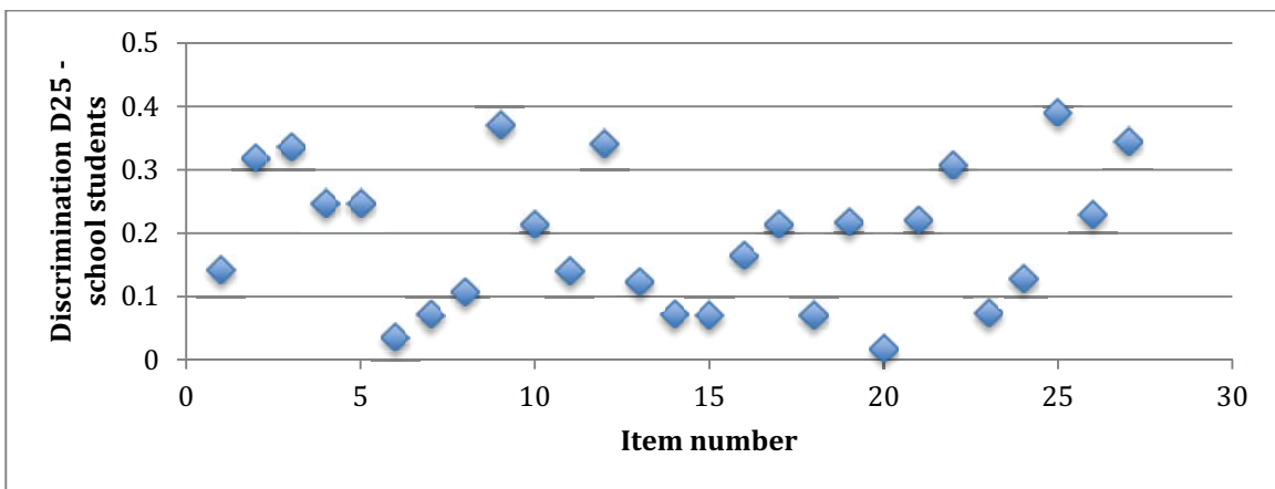
Figure 23: Item discrimination D_{25} for high school students
