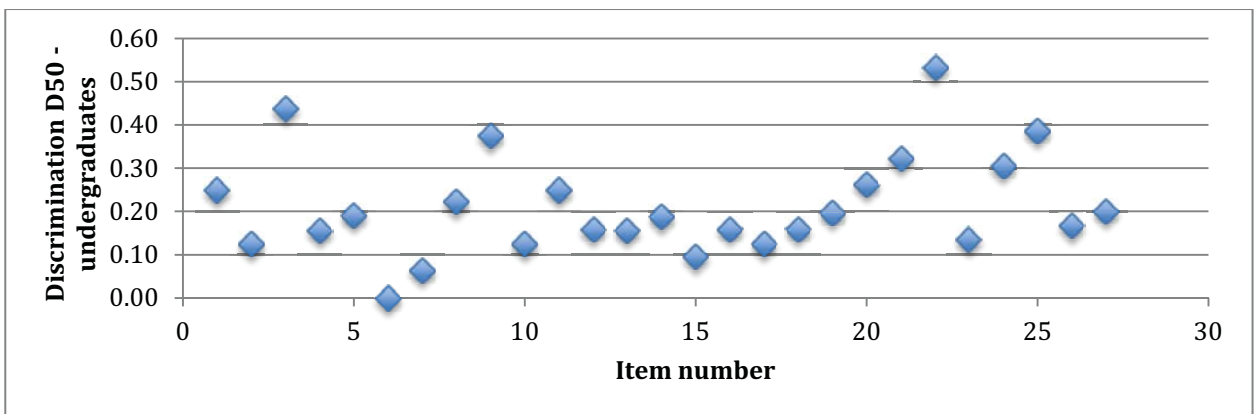
Figure 6: item discrimination D 50 for undergraduates
