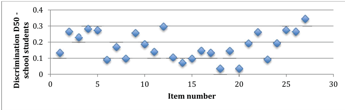
Figure 2: Item discrimination D_{50} for high school students
