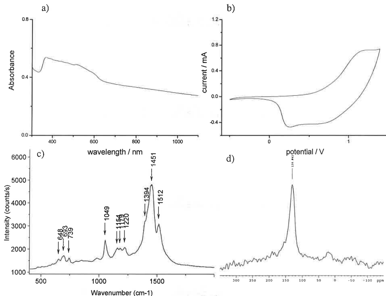
Figure 2. (a) UV-vis spectrum, (b) cyclic voltammogram, (c) Raman spectrum, and (d) ^{13}\text{C} CP-MAS solid-state NMR spectra of the poly(terthiophene) fibrils formed using the biphasic ionic liquid/water system.
