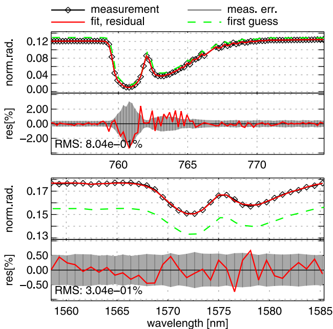
Figure 1. O 2 and CO 2 fit windows with SCIAMACHY measurements, first guess, fitted Sun-normalized radiation, residual, and measurement error for an exemplary SCIAMACHY pixel over Park Falls taken at 20 April 2007.
