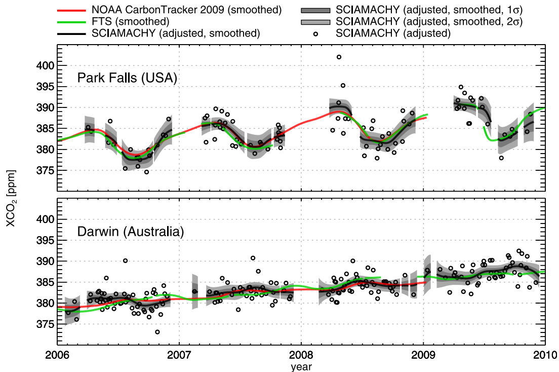
Figure 3. Smoothed representations of the time series measured at Park Falls and Darwin. The smoothing is performed by convolving the time series of Figure 2 with a Hann function with an effective width of 2 months (4 months in total). The gray shaded areas represent the standard error ( 1\sigma and 2\sigma ).
