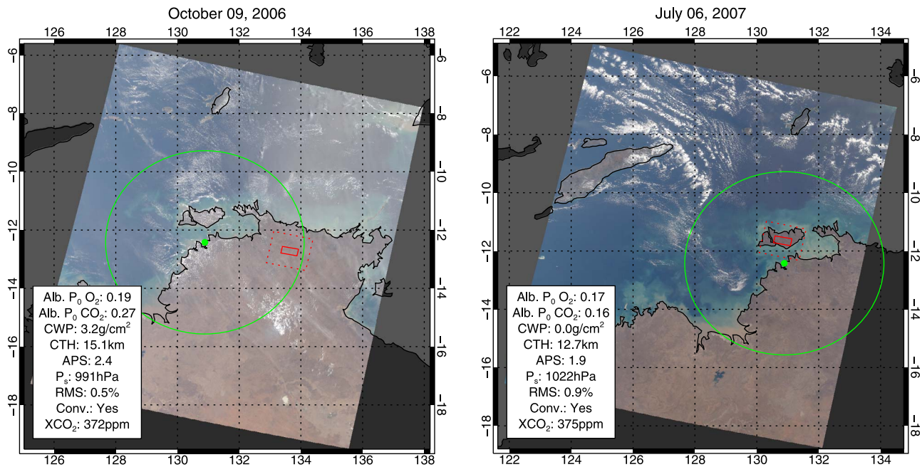
Figure 6. Meteorological situation of two exemplary SCIAMACHY measurements (red) falling in a 350 km surrounding of Darwin (green) as seen from MERIS. The SCIAMACHY pixels are encased by a 40 km cloud screening safety margin (red dotted box). (left) A typical cloud free situation. (right) In contrast to this, a situation with (undetected) cirrus clouds.
