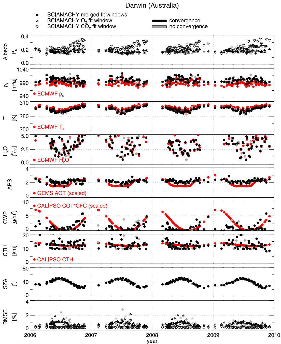
Figure 5. Darwin time series of selected important state vector elements which are byproducts of the SCIAMACHY XCO 2 retrieval. (top to bottom) Albedo in both fit windows represented by the zeroth-order polynomial, surface pressure, 2 m temperature, column-average mole fraction of water vapor, scaling factor for a default aerosol profile (APS), cloud water/ice content (CWP), cloud top height (CTP), solar zenith angle (SZA), and root mean square error of the fit residual in both fit windows. Corresponding values of ECMWF, CALIPSO (2007), and GEMS (2005) are also shown.
