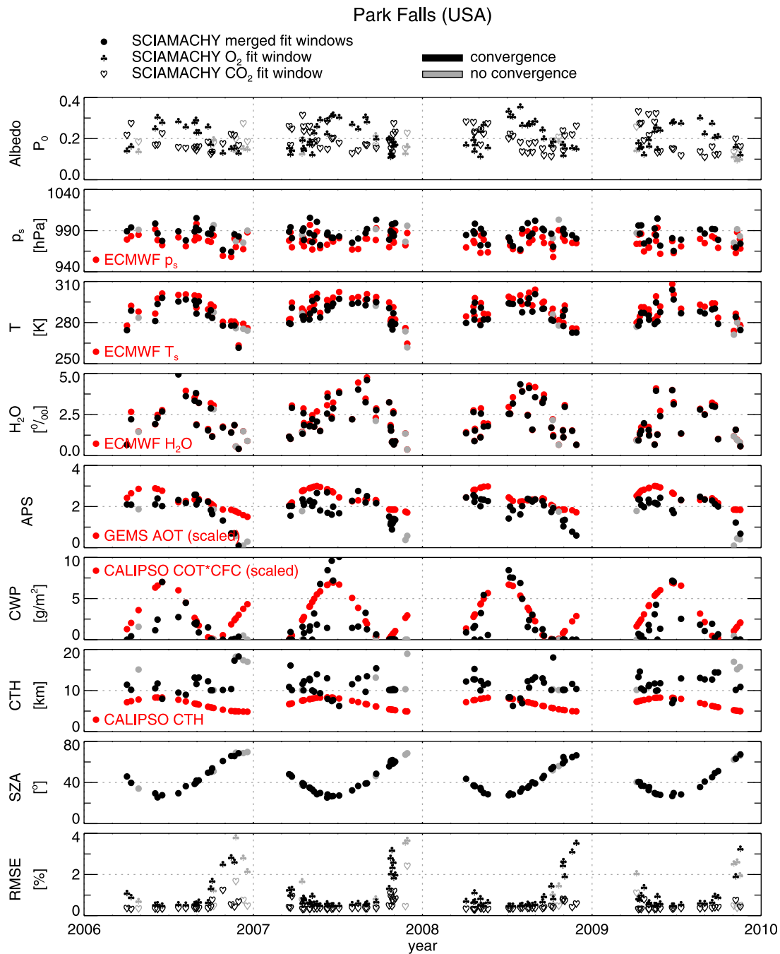
Figure 4. Park Falls time series of selected important state vector elements which are byproducts of the SCIAMACHY XCO 2 retrieval. (top to bottom) Albedo in both fit windows represented by the zeroth-order polynomial, surface pressure, 2 m temperature, column-average mole fraction of water vapor, scaling factor for a default aerosol profile (APS), cloud water/ice content (CWP), cloud top height (CTP), solar zenith angle (SZA), and root mean square error of the fit residual in both fit windows. Corresponding values of ECMWF, CALIPSO (2007), and GEMS (2005) are also shown.
