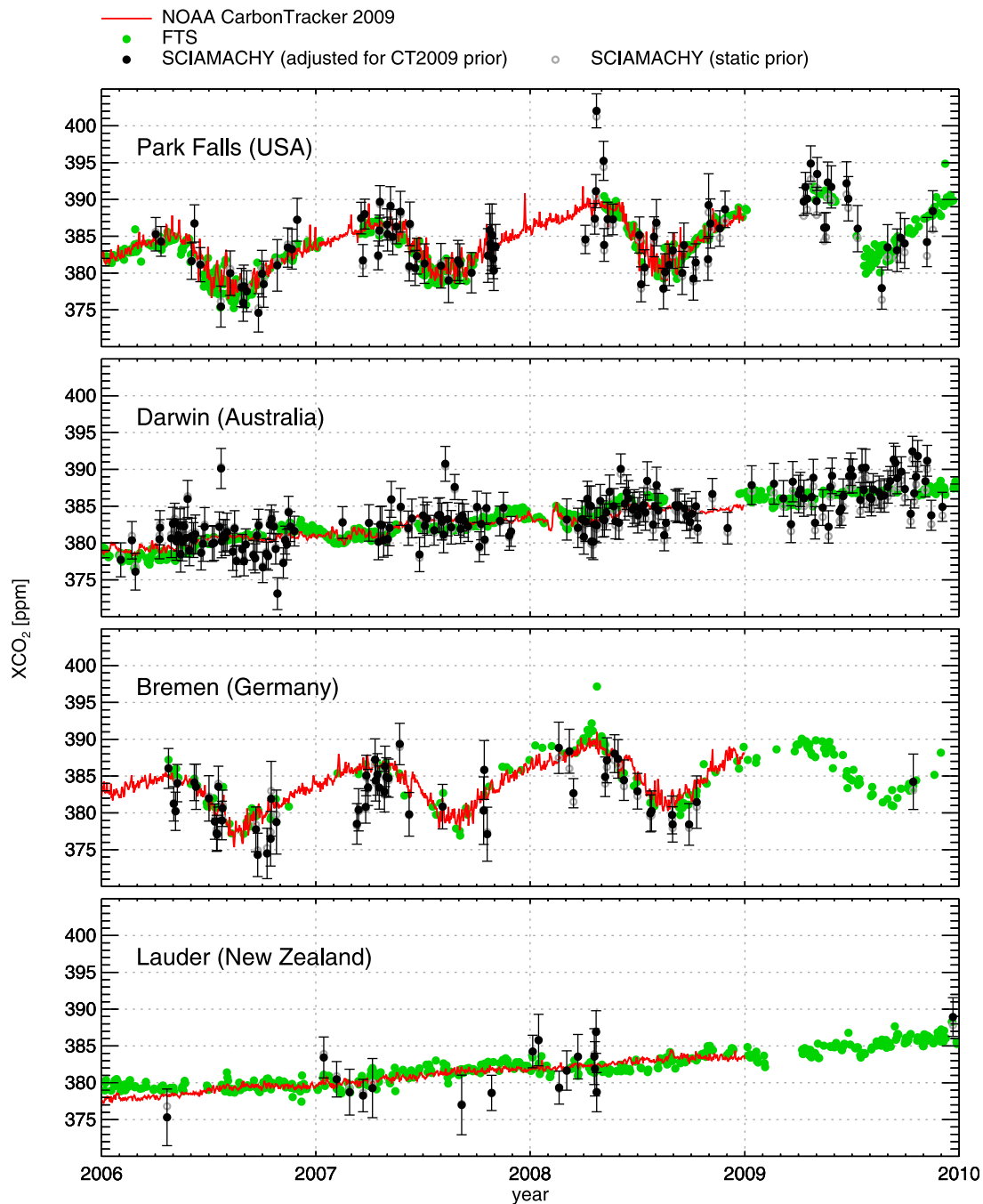
Figure 2. XCO 2 time series of individual measurements at the TCCON sites Park Falls, Darwin, Bremen, and Lauder. The corresponding statistical quantities which measure the agreement between the time series are given in Table 1.
