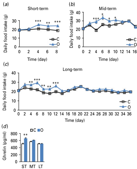
Fig. 1. Olanzapine increases daily food intake and plasma ghrelin levels in a time-dependent manner. In the short-term treatment cohort, daily food intake was increased by olanzapine from day four to day eight (a). In the mid-term treatment cohort, daily food intake was increased by olanzapine from day four to day ten (b). In the long-term cohort, daily food intake was increased by olanzapine from day four to day twelve (c). Olanzapine increased plasma ghrelin in the short-term cohort only (d). * p < 0.05 vs. Control; ** p < 0.01 vs. Control; *** p < 0.001 vs. Control; n = 10 –12 per treatment group.
