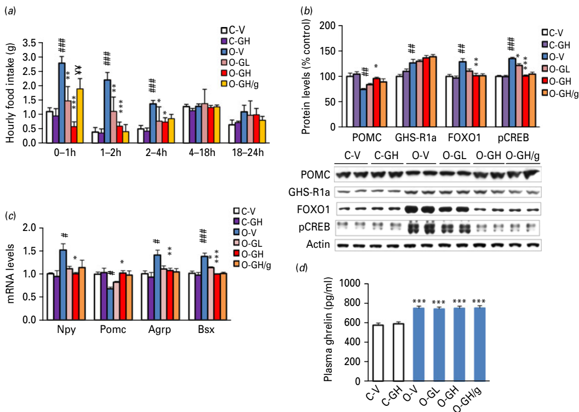
Fig. 7. Acute effects of olanzapine and the ghrelin receptor antagonist D-Lys3-GHRP-6 on food intake, plasma ghrelin levels, protein expressions of POMC, GHS-R1a, FOXO1 and pCREB, and mRNA levels of NPY, POMC, AgRP and BSX at the MBH. Olanzapine treatment produced a significant elevation effect on hourly food intake up to 4 h post-i.c.v. injection of vehicles, which was reduced or eliminated by i.c.v. injection of D-Lys3-GHRP-6 (3 nmol) or D-Lys3-GHRP-6 (30 nmol), respectively (a). Olanzapine decreased POMC, and increased FOXO1 and pCREB protein expressions at the MBH, which was eliminated by i.c.v. injection of D-Lys3-GHRP-6 (30 nmol) (b). Olanzapine increased GHS-R1a protein expressions at the MBH, which could not be reversed by D-Lys3-GHRP-6 (b). Olanzapine increased NPY, AgRP and BSX, but decreased POMC mRNA expressions at the MBH, which were eliminated by i.c.v. injection of D-Lys3-GHRP-6 (30 nmol) ( p < 0.05 ; n = 6 ) (c). Plasma ghrelin levels were increased by oral olanzapine treatment (d). This effect was not affected by i.c.v. injection of D-Lys3-GHRP-6 (3 nmol) or D-Lys3-GHRP-6 (30 nmol) ( d ) ^{\#}p < 0.05 vs. C-V; ^{\#\#}p < 0.01 vs. C-V; ^{\#\#\#}p < 0.001 vs. C-V; ^*p < 0.05 vs. O-V; ^{**}p < 0.01 vs. O-V; ^{***}p < 0.001 vs. O-V; ^{yy}p < 0.01 vs. O-GH; n = 5-6 per treatment group. C-V: the oral control and ICV vehicle group; C-GH: the oral control and i.c.v. high-dose GHS-R1a antagonist group; O-V: the oral olanzapine and ICV vehicle group; O-GL: the oral olanzapine and i.c.v. low-dose GHS-R1a antagonist group; O-GH: the oral olanzapine and high-dose GHS-R1a antagonist group; O-GH/g: the oral olanzapine and i.c.v. high-dose GHS-R1a antagonist with ghrelin co-treatment group.
