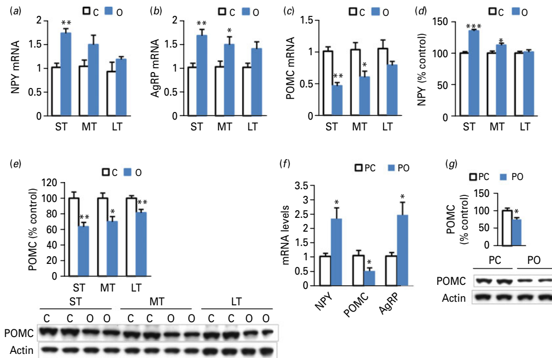
Fig. 5. Effects of olanzapine on hypothalamic expressions of neuropeptides NPY, POMC and AgRP. Olanzapine increased hypothalamic NPY mRNA expressions in the short-term only (a). Olanzapine increased hypothalamic AgRP mRNA expressions in the short- and mid- term, but not in the long-term (b). Olanzapine reduced hypothalamic POMC mRNA expressions in the short- and mid-term (c). Olanzapine increased hypothalamic NPY protein expressions in the short- and mid- term, as detected by EIA (d). Olanzapine decreased hypothalamic POMC protein expressions in the short-, mid- and long-term, as detected by Western blot (e). Pair-fed olanzapine treatment increased hypothalamic mRNA expressions of NPY and AgRP, but decreased POMC mRNA expressions (f). Pair-fed olanzapine treatment down-regulated hypothalamic POMC protein expressions (g). * p < 0.05 vs. Control; ** p < 0.01 vs. Control; *** p < 0.001 vs. Control; n = 5-6 per treatment group.
