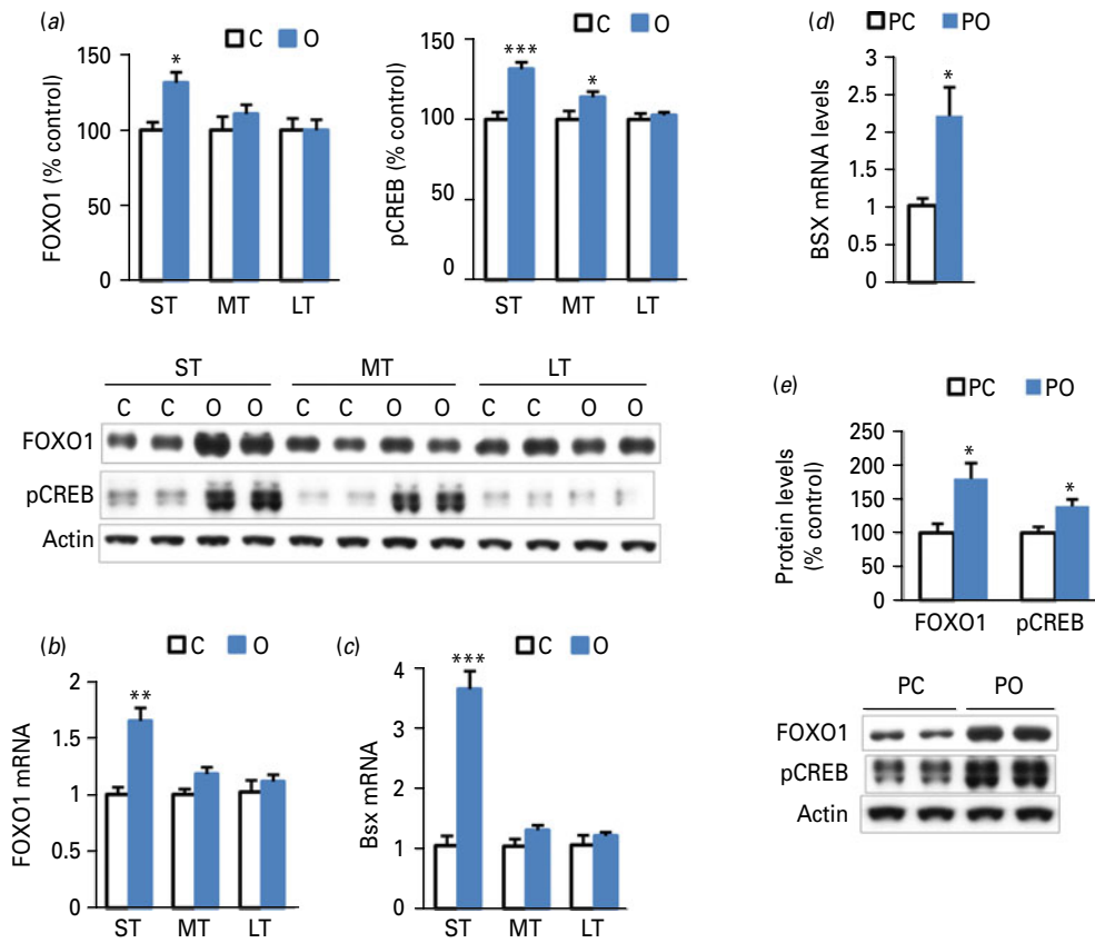
Fig. 6. Effects of olanzapine on hypothalamic FOXO1, pCREB, and BSX expressions. Olanzapine increased hypothalamic FOXO1 protein expressions in the short-term only, while increasing hypothalamic pCREB protein expressions in the short- and mid-term (a). Olanzapine increased hypothalamic FOXO1 and BSX mRNA expressions in the short-term only (b; c). Pair-fed olanzapine treatment increased hypothalamic BSX mRNA expressions (d). Pair-fed olanzapine treatment increased hypothalamic FOXO1, and pCREB protein expressions (e) * p < 0.05 vs. Control; ** p < 0.01 vs. Control; *** p < 0.001 vs. Control; n = 5-6 per treatment group.
