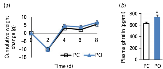
Fig. 3. Effects of pair-fed olanzapine treatments on cumulative weight change and circulating ghrelin levels. Pair-fed olanzapine treated rats had no significant weight change difference compared to the pair-fed control group (a). Pair-fed olanzapine treated rats had elevated plasma ghrelin levels compared to the pair-fed control group (b). * p < 0.05 vs. Pair-fed Control; n = 12 per treatment group.
