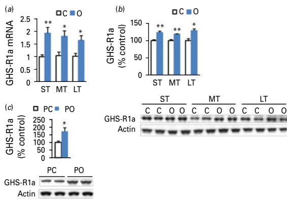
Fig. 4. Effects of olanzapine treatments on hypothalamic GHS-R1a mRNA and protein expressions. Olanzapine increased hypothalamic GHS-R1a mRNA levels in the short-, mid- and long-term as detected by qRT-PCR (a). Olanzapine increased hypothalamic GHS-R1a protein levels in the short-, mid- and long-term as detected by Western blot (b). Pair-fed olanzapine treatment increased hypothalamic GHS-R1a protein expressions (c). * p < 0.05 vs. Control; ** p < 0.01 vs. Control; n = 5-6 per treatment group.
