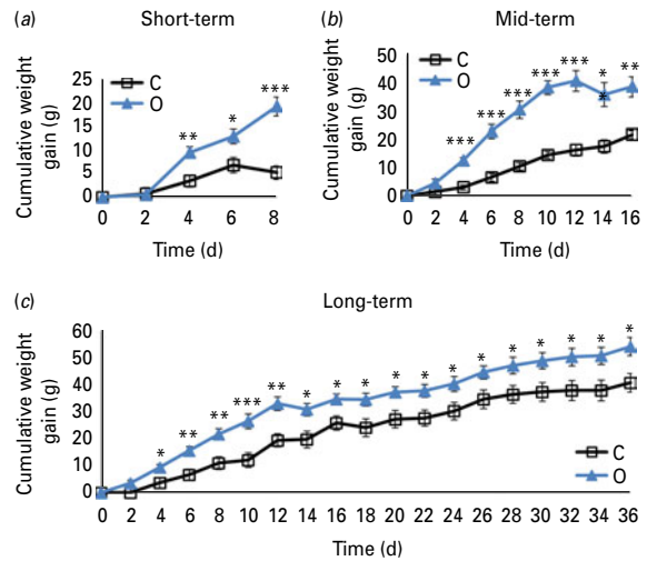
Fig. 2. Olanzapine increases cumulative body weight gain. Cumulative body weight gain was increased by olanzapine from day four of treatment in the short-term (a), mid-term (b) and long-term (c) cohorts. * p < 0.05 vs. Control; ** p < 0.01 vs. Control; *** p < 0.001 vs. Control; n = 10 –12 per treatment group.
