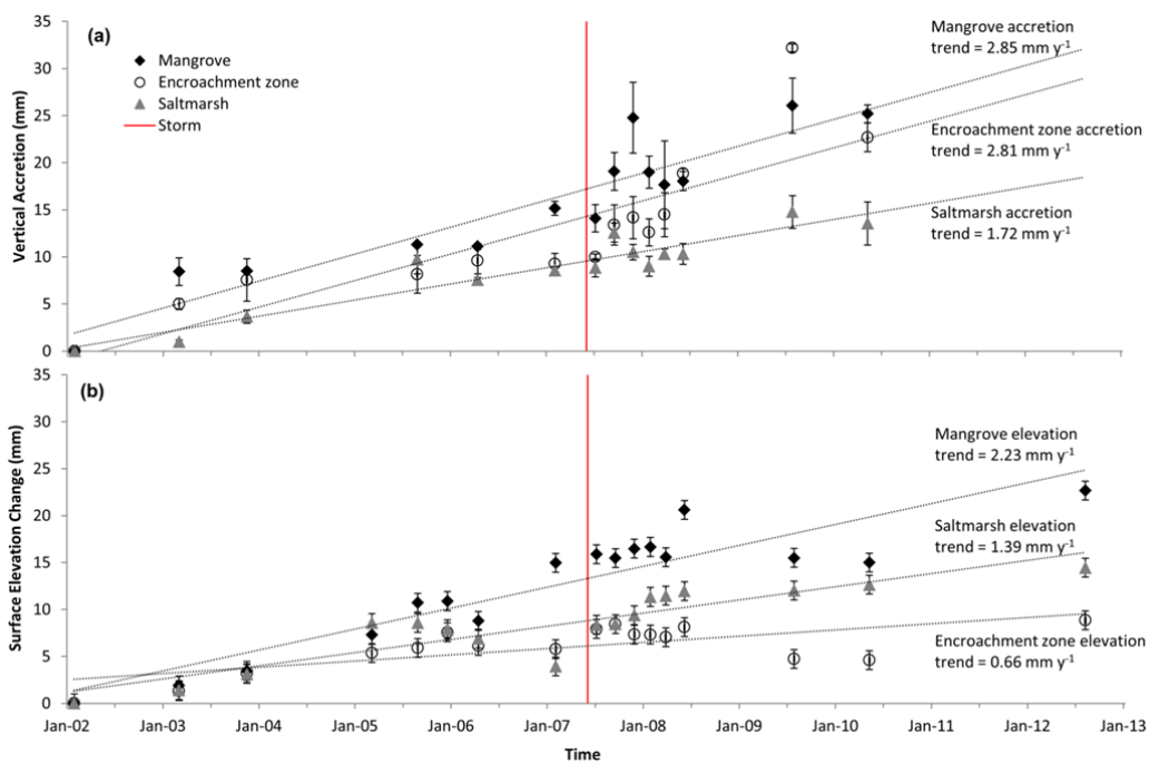
Figure 4: Accretion and elevation trends for mangrove, salt marsh and mangrove encroachment zones at Kooragang Island. (a) Vertical accretion, and (b) surface elevation change. The storm event is indicated by a red vertical line in (a) and (b).
