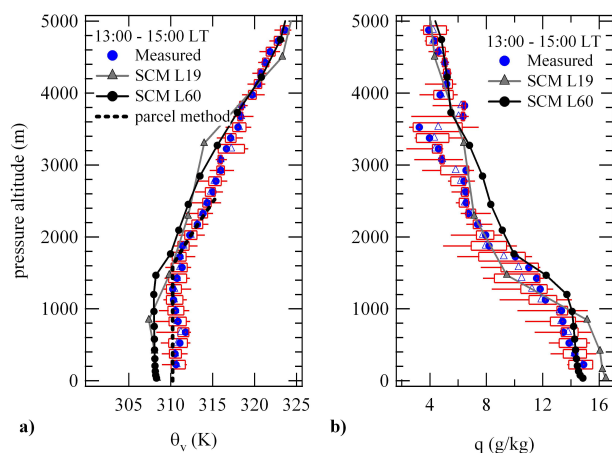
Fig. 3. Virtual potential temperature and specific humidity profiles between 13:00 and 15:00 gathered from several flights above the Guyana's rainforest in comparison to their SCM simulated profiles.
