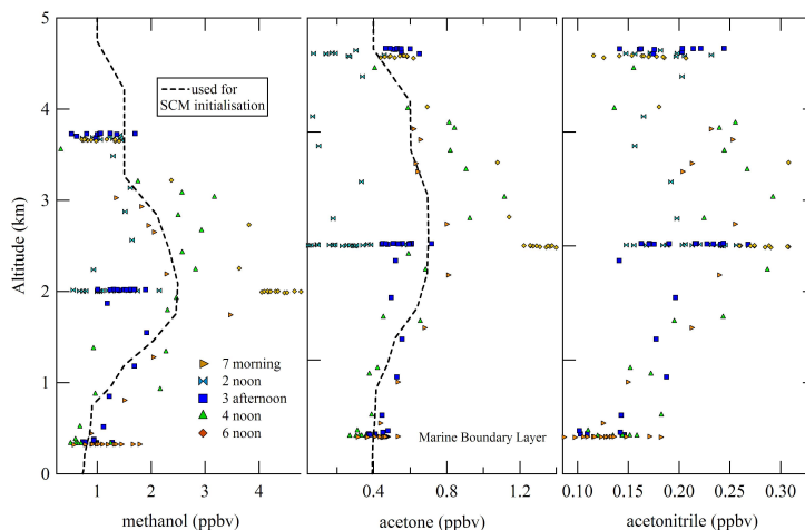
Fig. 2. Oceanic vertical profiles for methanol, acetone and acetonitrile used for SCM-model initialisation.
