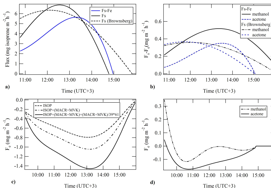
Fig. 11. (a and b) Comparison of the mixed layer median fluxes for isoprene (after correction for chemical loss), methanol and acetone to their surface layer fluxes obtained for Brownsberg. (c and d) Estimated entrainment fluxes based on the concentration jump method.
