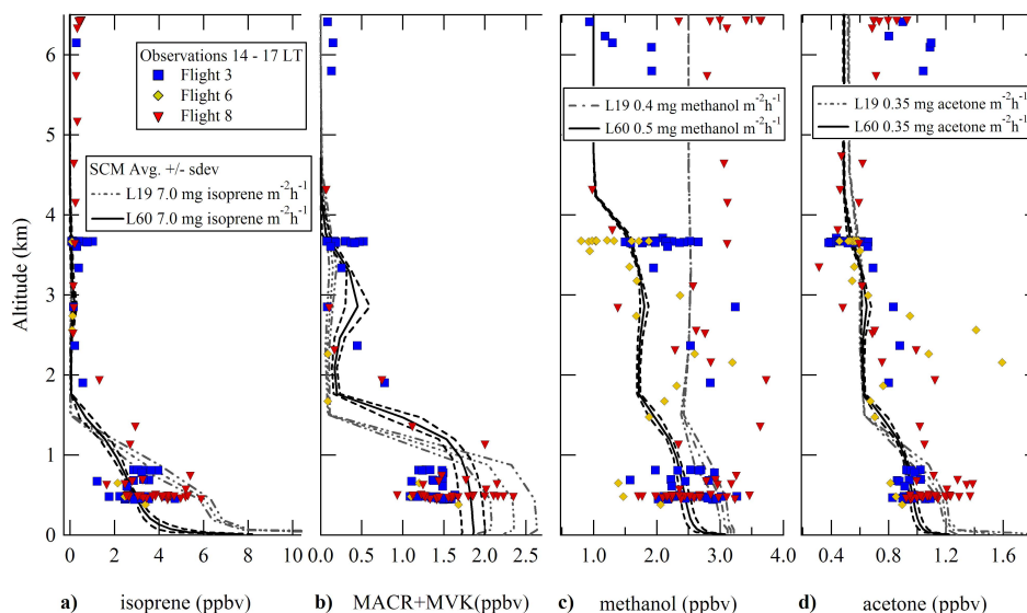
Fig. 6. Measured and modelled vertical profiles for isoprene, the sum of methacrolein and methyl vinyl ketone, methanol and acetone over the rainforest for the first day over land.
