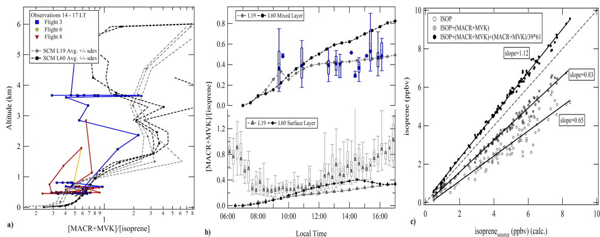
Fig. 10. Comparison of the measured to the modelled vertical (14:00–17:00 LT) and diurnal cycle of [MACR+MVK]/[isoprene] (first day over land). Comparison of compensation for chemical loss of isoprene (see text).
