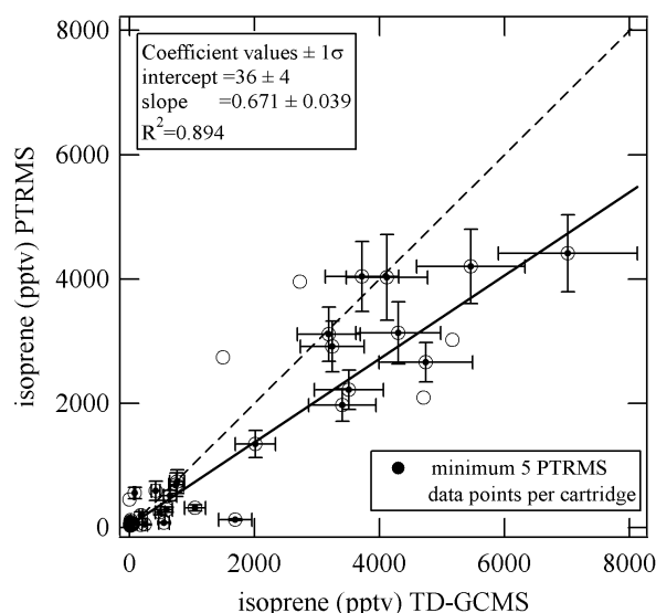
Fig. 1. Orthogonal distance regression of PTR-MS vs. TD-GCMS. Error bars represent the total measured uncertainty for each measurement technique within each interval of comparison.
