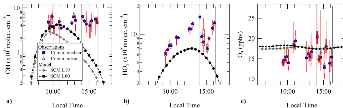
Fig. 9. Measured and modelled diurnal cycles of OH, HO 2 and O 3 above the rainforest for October 2005.
