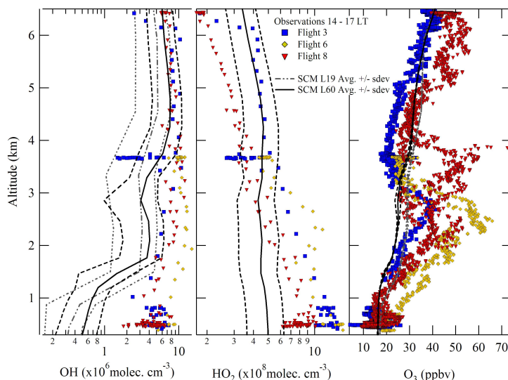
Fig. 7. Measured and modelled vertical profile of OH, HO 2 and O 3 over the Tropical rainforest.
