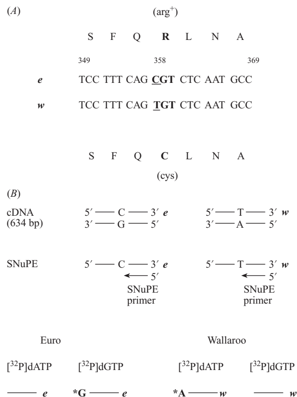
Fig. 1. Single Nucleotide Primer Extension (SNuPE) assay for allele-specific G6PD expression in M. robustus cDNA. (A) Comparison of G6PD cDNA sequence (exon 5, position 349–369) showing the base difference between M. r. robustus ( w = wallaroo) and M. r. erubescens ( e = euro). (B) In the SNuPE assay, [ 32 P]dATP is specific for the wallaroo allele as it is complementary to T (the base next to the SNuPE primer), and [ 32 P]dGTP is specific for the euro allele, being complementary to the next base C. The product, after one PCR cycle, consisted of the SNuPE primer and the allelic specific radioactive nucleotide added. ( w , wallaroo; and e , euro; *, band present).
