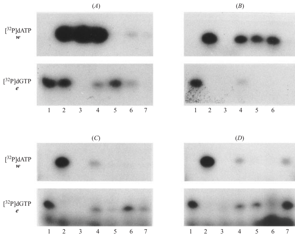
Fig. 2. Allele-specific expression of G6PD in different cell types of M. robustus . The top row of bands represents expression detected by the radioactive nucleotide [ ^{32}\text{P} ]dATP, which is specific for the wallaroo ( w ) allele, and the lower row represents expression detected by [ ^{32}\text{P} ]dGTP, which is specific for the euro ( e ). (A) Controls, top row: lanes (1) no cDNA; (2) 5 ng e plus 5 ng w cDNA; (3) 10 ng w cDNA. Controls, lower row: lanes (1) 10 ng e cDNA; (2) 5 ng e plus 5 ng w cDNA; (3) no cDNA. Samples: lanes (4) we hybrid cultured fibroblasts; (5) e cultured fibroblasts; (6) ew hybrid cultured fibroblasts; (7) w cultured fibroblasts. (B) Controls, top row: lanes (1) no cDNA; (2) 10 ng w cDNA; (3) 10 ng e cDNA. Controls, lower row: lanes (1) 10 ng e cDNA, (2) no cDNA, (3) 10 ng w cDNA. Samples: lanes (4) we hybrid cultured fibroblasts; (5) we ovary (6) we uterus. (C) Controls: lanes (1)–(3) as in (B). Samples: lanes (4) ew hybrid cultured fibroblasts; (5) ew kidney; (6) ew brain; (7) ew heart. (D) Controls: lanes (1)–(3) as in (B). Samples: lanes (4) ew hybrid cultured fibroblasts; (5) ew liver; (6) blastocyst (unsexed); (7) ew oocytes.
