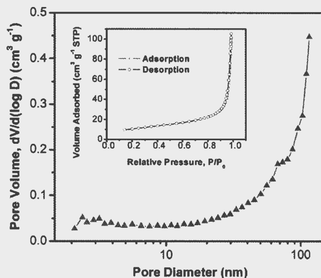
Figure 3. (Color online) Pore size distribution curve of the FSP-made \text{LiV}_3\text{O}_8 nanoparticles, calculated from the adsorption points using the BJH algorithm. Inset shows the corresponding \text{N}_2 adsorption–desorption isotherms.
