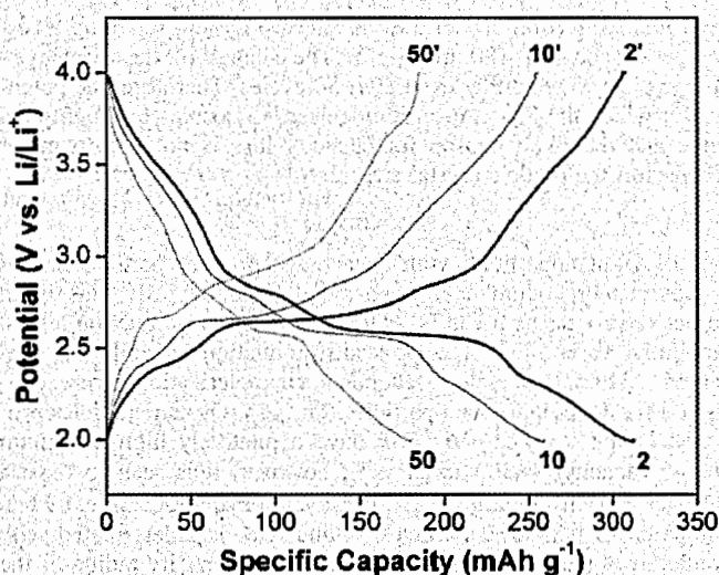
Figure 6. (Color online) Second, tenth, and 50th cycle discharge-charge plots of \text{LiV}_3\text{O}_8 electrode. Cycling took place between 2.0 and 4.0 V vs \text{Li}/\text{Li}^+ at 100 \text{ mA g}^{-1} .
