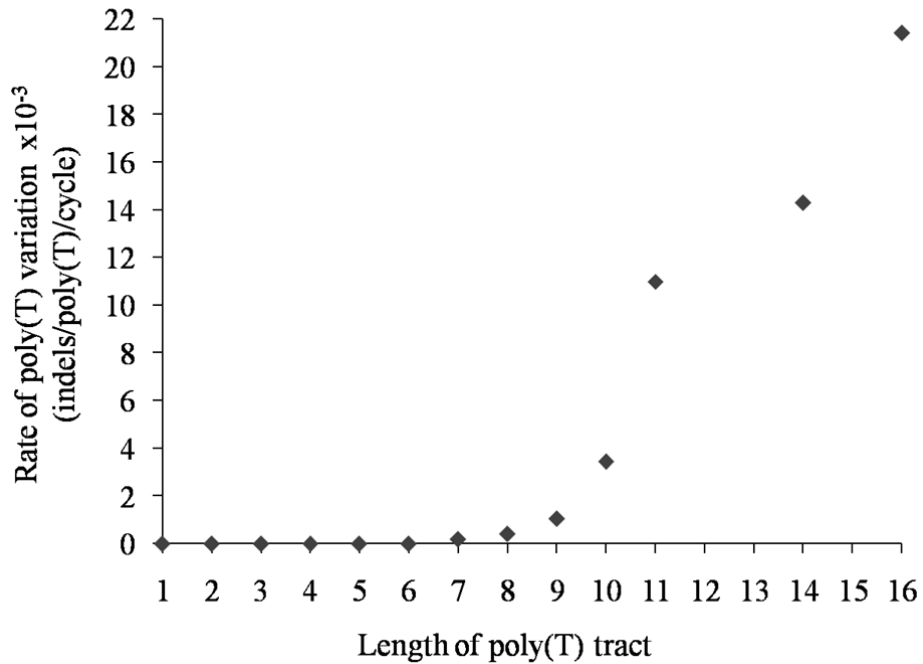
Figure 2 Relationship between the rate of poly(T) variation and poly(T) tract length of all indel types in COI and COII for all Hoplolaimoidea species studied.
