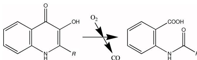
Figure 1 The reactions catalysed by QDO ( R = H ) and HOD ( R = CH_3 ). The substrates are 1 H -3-hydroxy-4-oxoquinoline ( R = H ) and 1 H -3-hydroxy-4-oxoquinoline ( R = CH_3 ).
