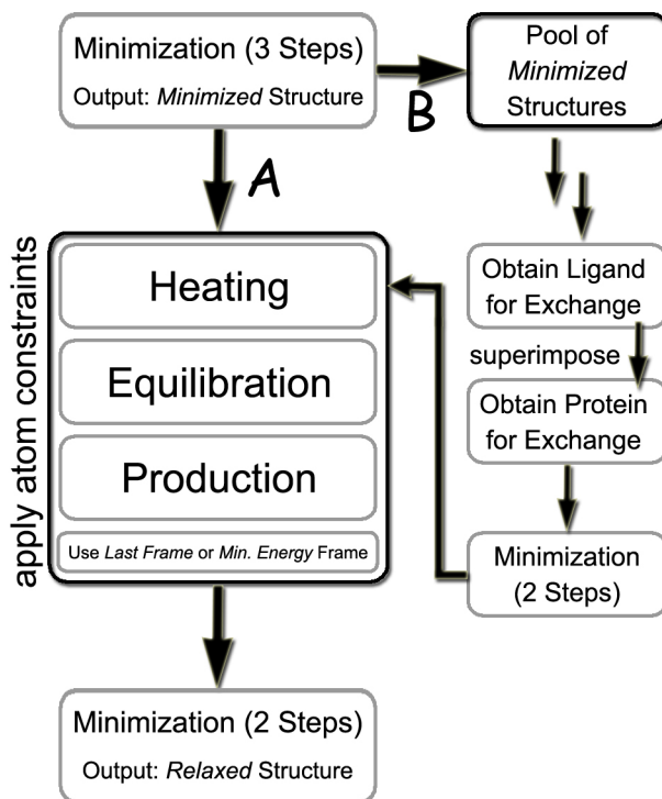
Scheme 1: Flow diagram summarizing the modelling protocols employed. The protocol for the relaxation of the crystal structures proceeded via path A , while the protocol for the ligand exchange simulations proceeded via path B .
