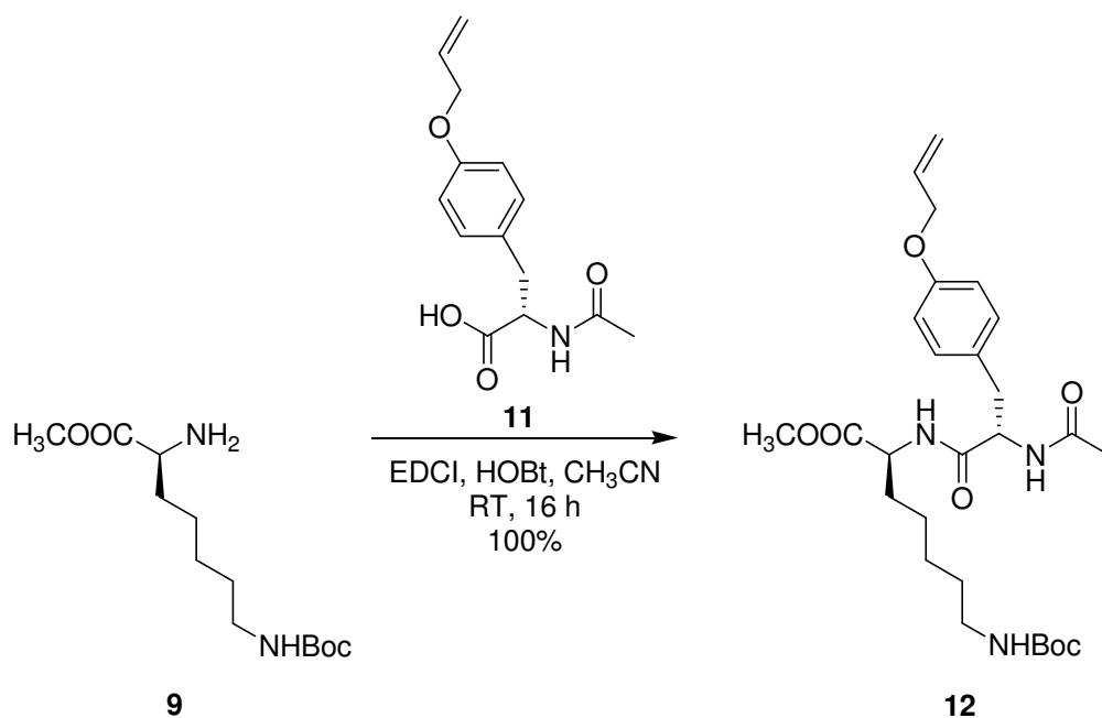
Scheme 2: Synthesis of the diastereomeric dipeptide 12 .
