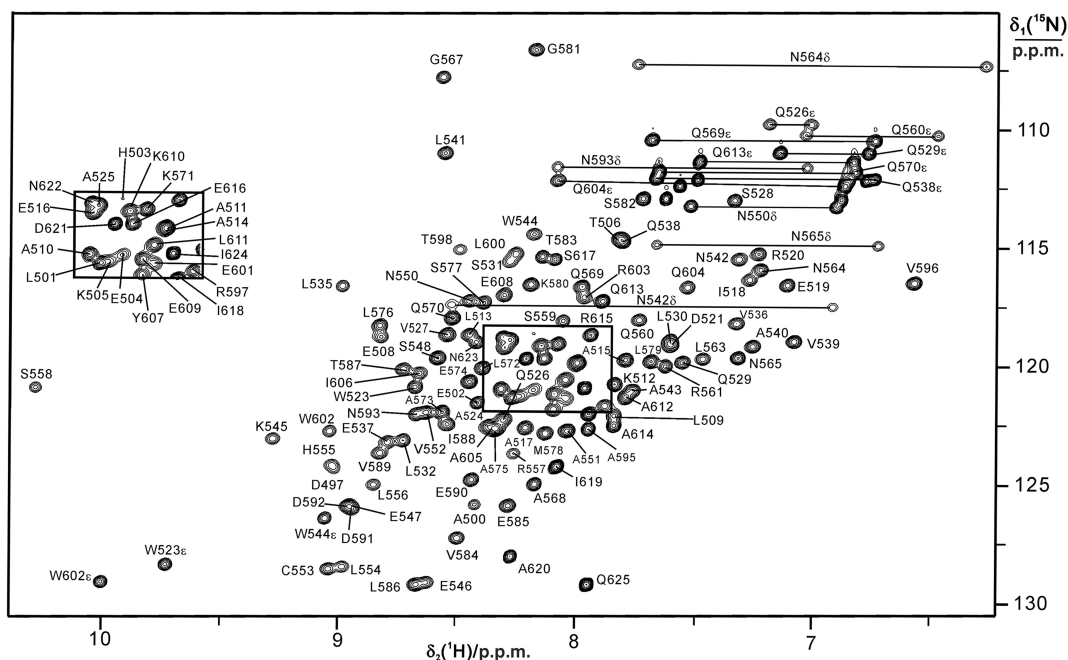
Figure 2. ^{15}\text{N} -HSQC spectrum of \tau_{\text{C14}} . The spectrum was recorded at 30^\circ\text{C} with a 1.8 mM solution of uniformly ^{15}\text{N}/^{13}\text{C} -labeled \tau_{\text{C14}} in 90% \text{H}_2\text{O}/10\% \text{D}_2\text{O} at pH 6.8 in phosphate buffer (10 mM phosphate, 100 mM NaCl, 1.0 mM dithiothreitol and 0.1 mM \text{NaN}_3 ). The cross-peaks are assigned using one-letter amino acid symbols and residue numbers. Side-chain resonances are identified by Greek characters. Cross-peaks from side-chain amides are connected by horizontal lines.
