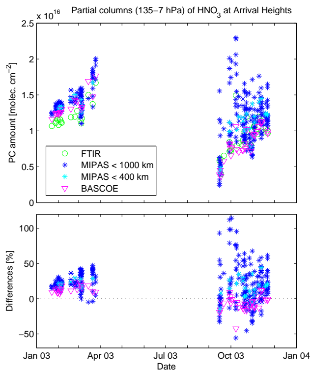
Fig. 10. Upper panel: Partial columns (135–7 hPa) of HNO 3 at Arrival Heights, from ground-based FTIR (green circles), MIPAS (dark blue and light blue stars for selections according to the spatial collocation criteria of 1000 and 400 km, respectively) and BASCOE (magenta triangles) data. Lower panel: Relative partial column differences (MIPAS-FTIR)/<FTIR> (stars; same colour coding as for upper plot), and (BASCOE-FTIR)/<FTIR> (magenta triangles).
