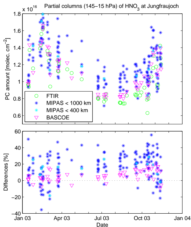
Fig. 11. Upper panel: Partial columns (145–15 hPa) of HNO 3 at the Jungfraujoch, from ground-based FTIR (green circles), MIPAS (dark blue and light blue stars for selections according to the spatial collocation criteria of 1000 and 400 km, respectively) and BASCOE (magenta triangles) data. Lower panel: Relative partial column differences (MIPAS-FTIR)/<FTIR> (stars; same colour coding as for upper plot), and (BASCOE-FTIR)/<FTIR> (magenta triangles).
