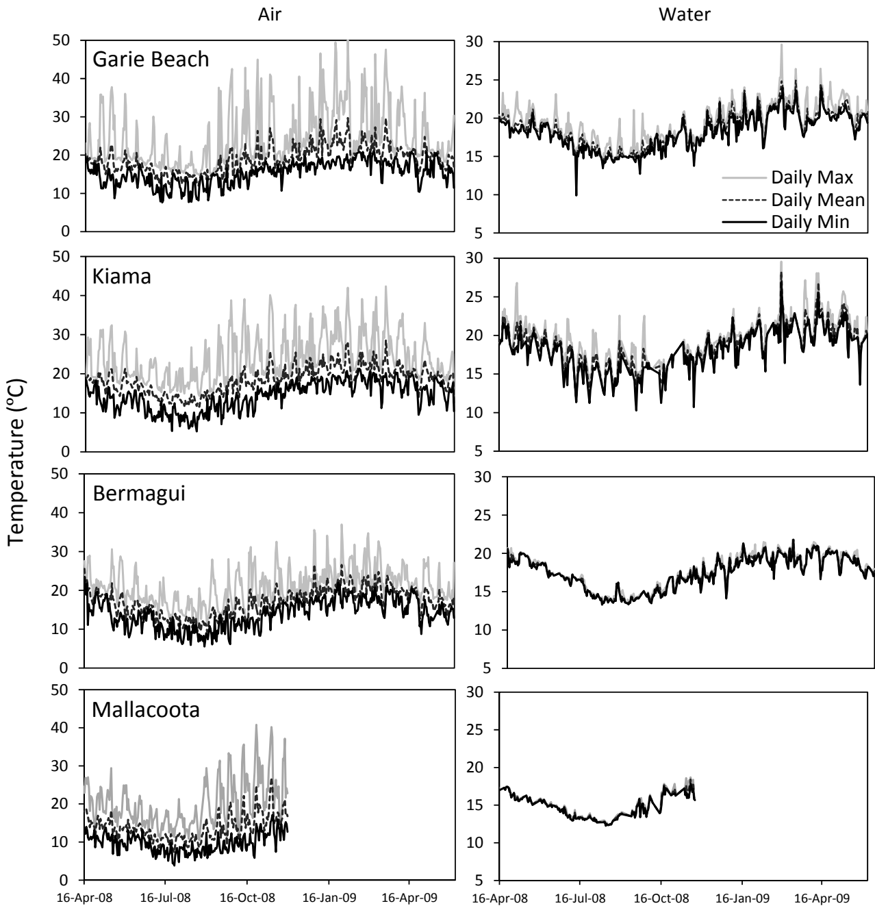
Fig. 2. Daily mean, maximum and minimum air and water temperatures recorded by in situ data loggers at the 4 study locations from the 16 April 2008 to 6 June 2009 (Mallacoota data only till 10 December 2008). Note different scales on y-axis.
