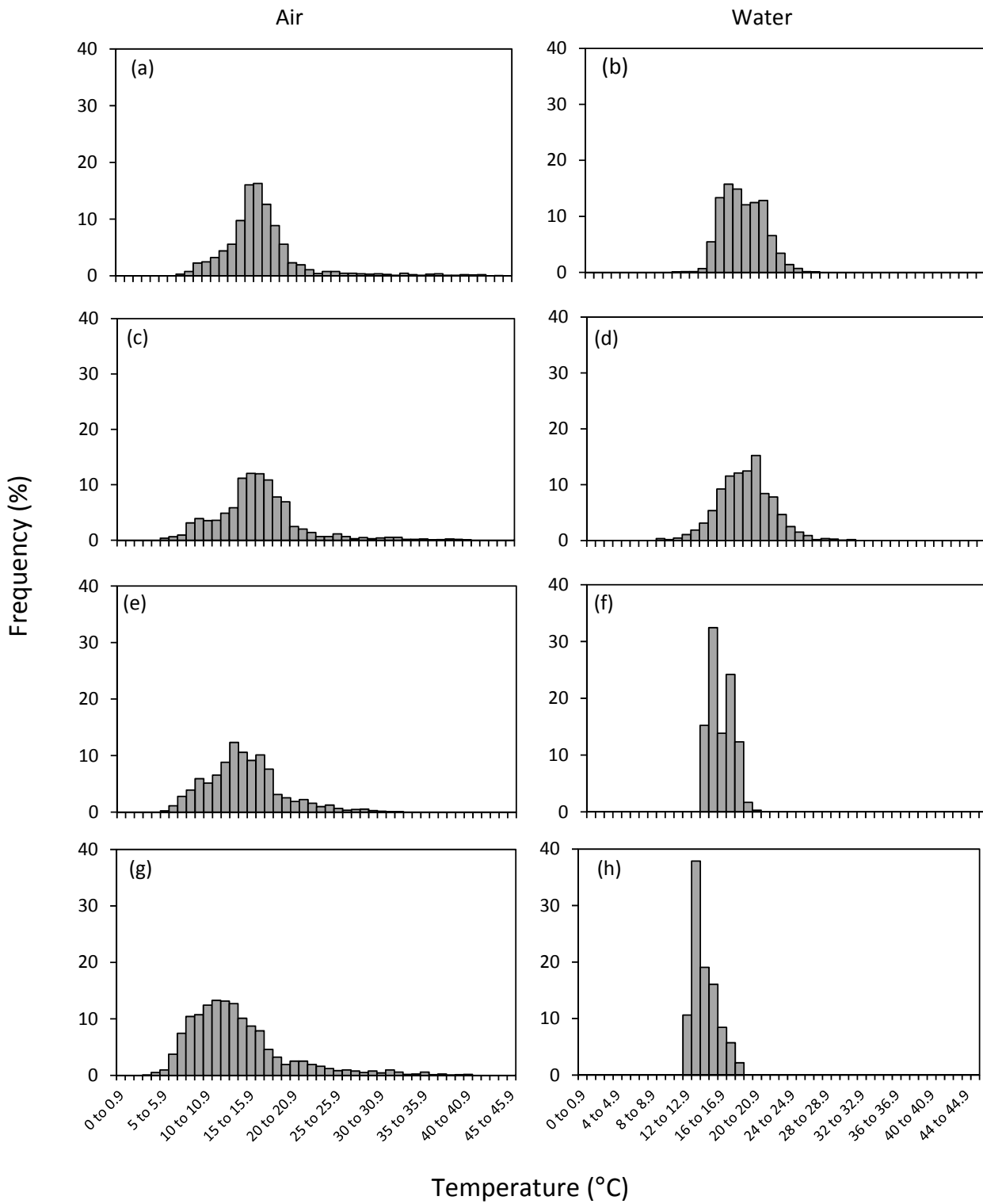
Fig. 3. In situ logger air and water temperature frequency distributions at Garie Beach (a-b), Kiama (c-d), Bermagui (e-f) and Mallacoota (g-h) from 1 June to 30 November 2008. Locations are arranged from north to south.
