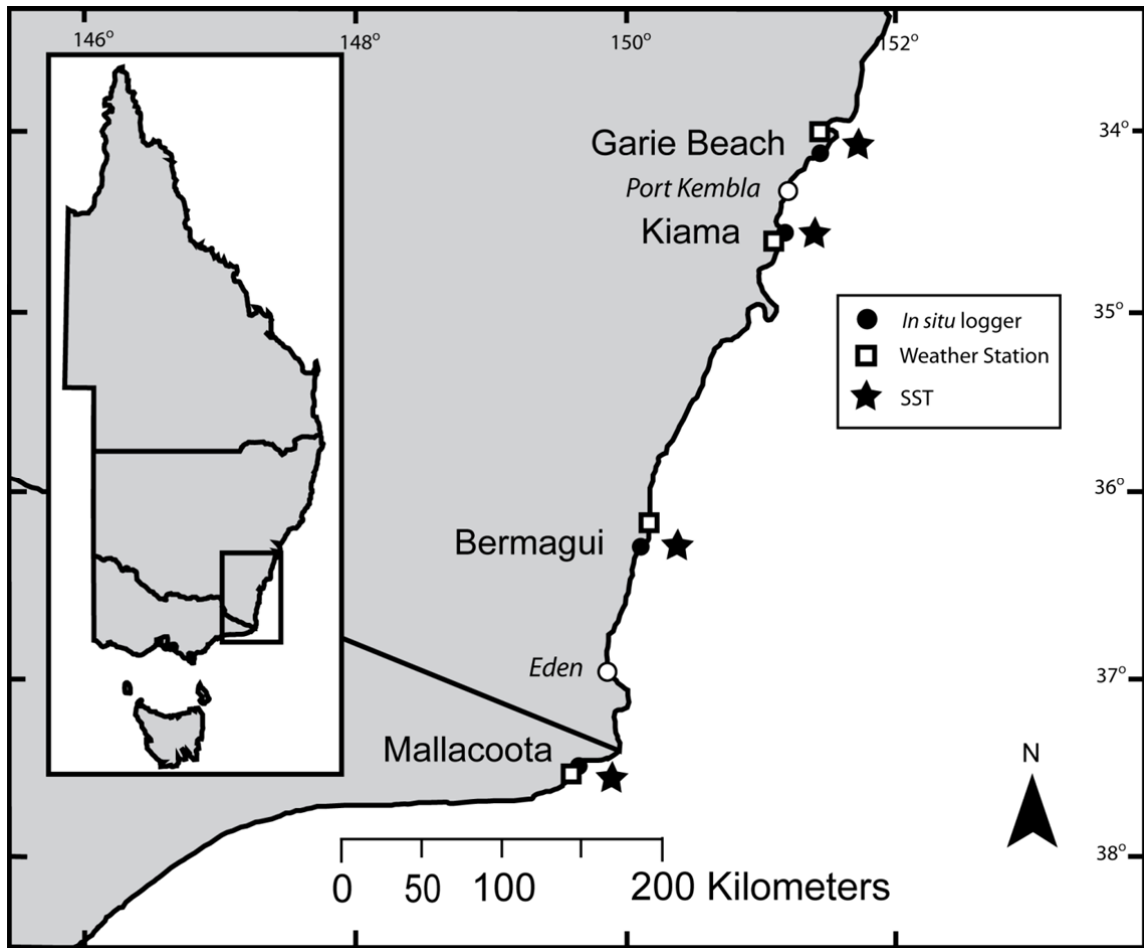
Fig. 1. Map of the 4 rocky intertidal shores along the southeast coast of Australia showing approximate locations of in situ logger, weather station and satellite sea surface temperature (SST) collection points. Port Kembla and Eden represent locations where tidal data was obtained.
