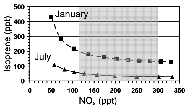
Fig. 6. Required isoprene mixing ratios for varying \text{NO}_x concentrations to match HCHO observations in January and July at Lauder, same symbols as in Fig. 8. The shaded area represents likely \text{NO}_x concentrations at Lauder (see Sect. 5).
