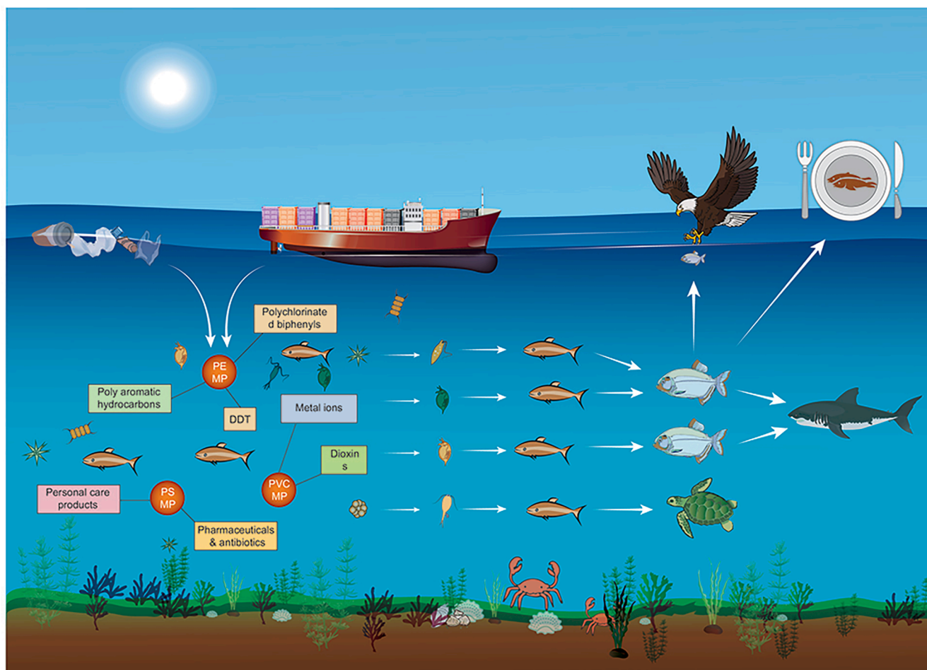
Fig. 4. Trophic transfer possibilities of microplastic-bound PPCP compounds and other contaminants in the ecosystem.
