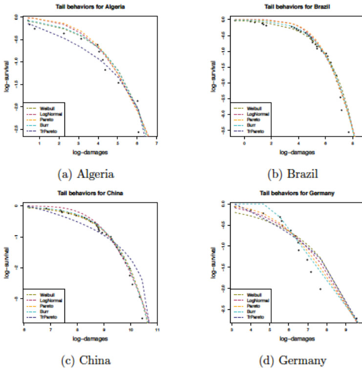
Figure 2: Log-log plots for fitting annual flood loss data by country. Black dots are observed values. Dashed curves are fitted parametric distributions.
