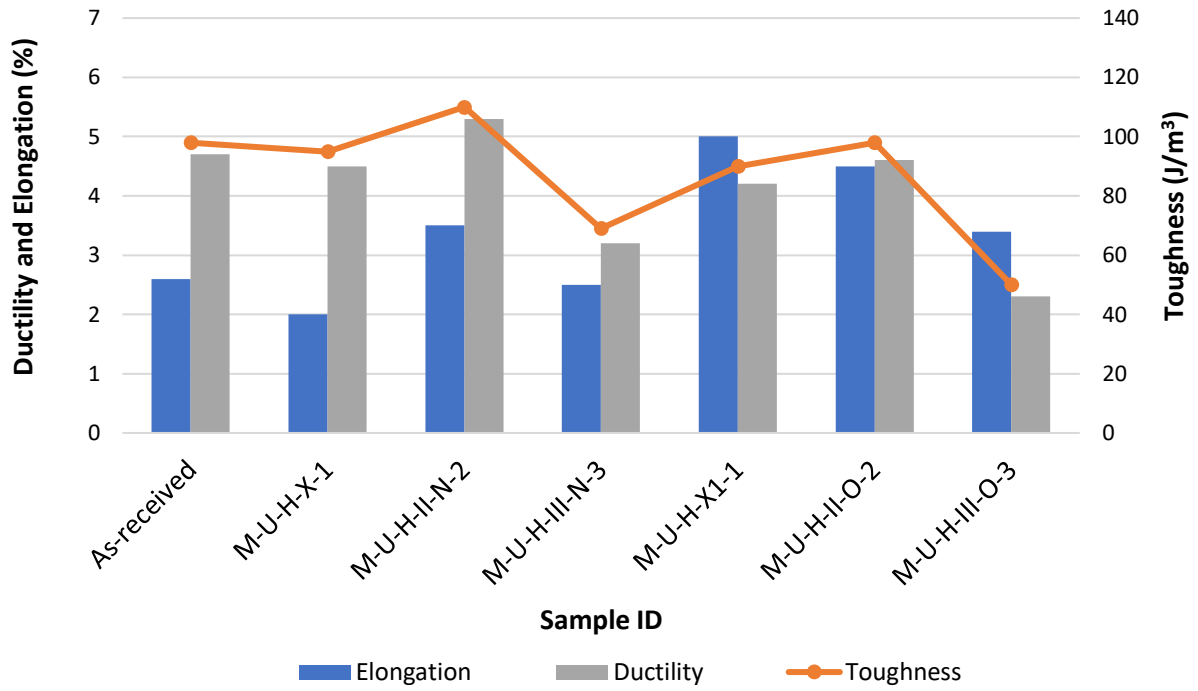
Figure 13 Comparison of ductility properties for tendons with High level of pre-stress exposed to ICCP-N & ICCP-O
