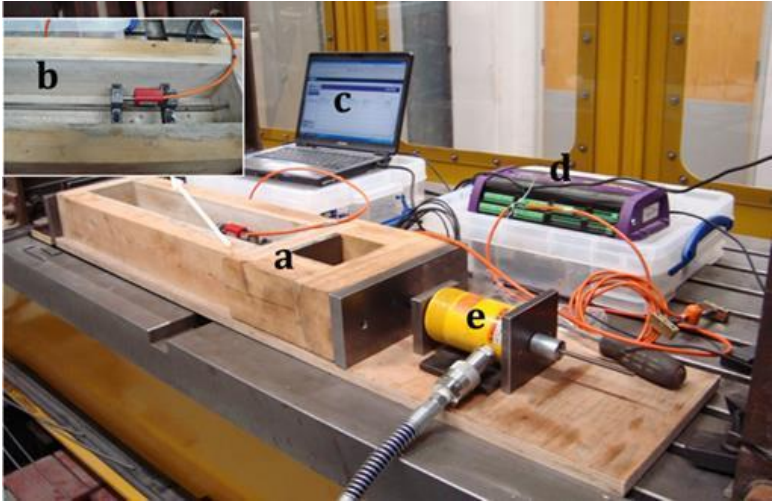
Figure 1 Pre-stressing System (a) mould; (b) strain gauge attached to pre-stressed tendon; (c) laptop; (d) data logger; (e) hydraulic jack connected to hand pump
