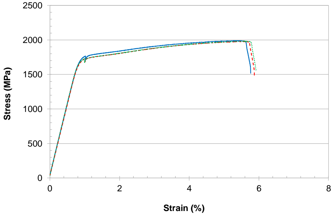
Figure 7 Stress-Strain curves for three as-received tendons
