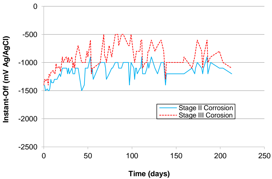
Figure 4 E_{off} for High pre-stressed tendons (Batch 4)
