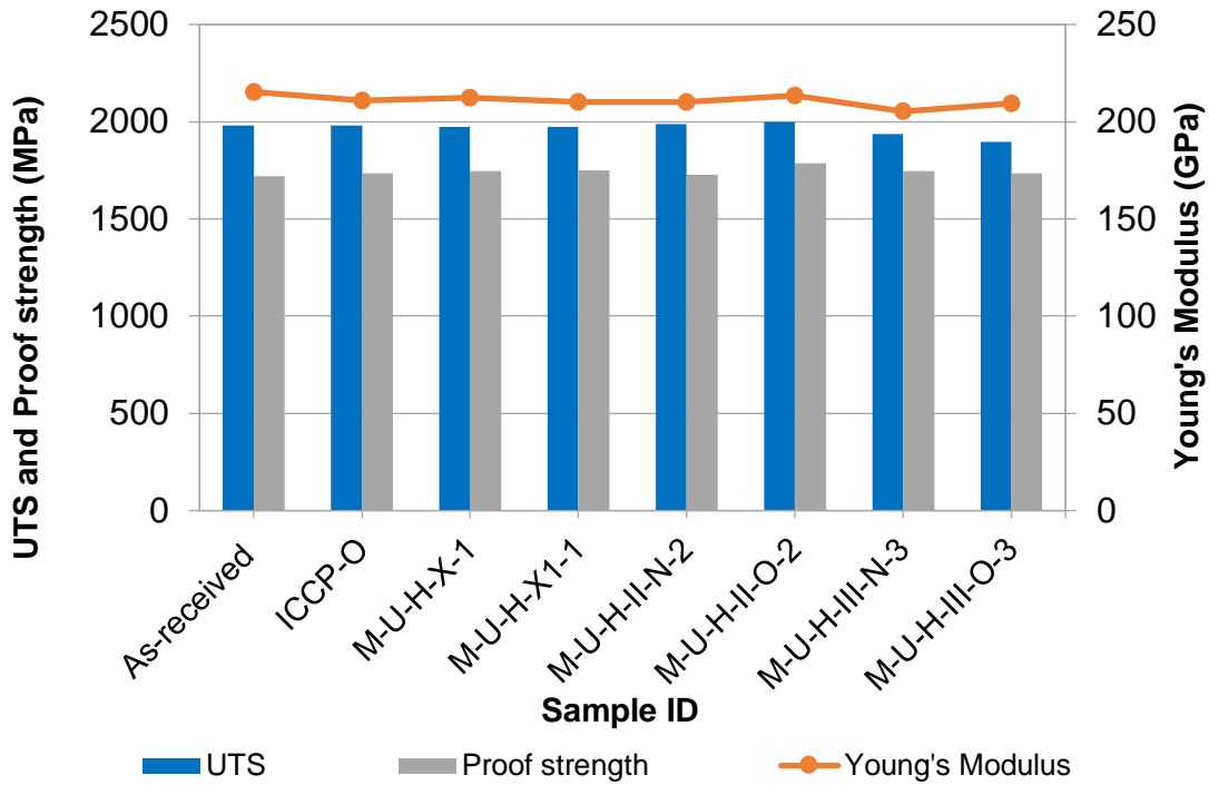
Figure 11 Comparison of mechanical properties for tendons with High Level of pre-stress exposed to ICCP-N & ICCP-O
