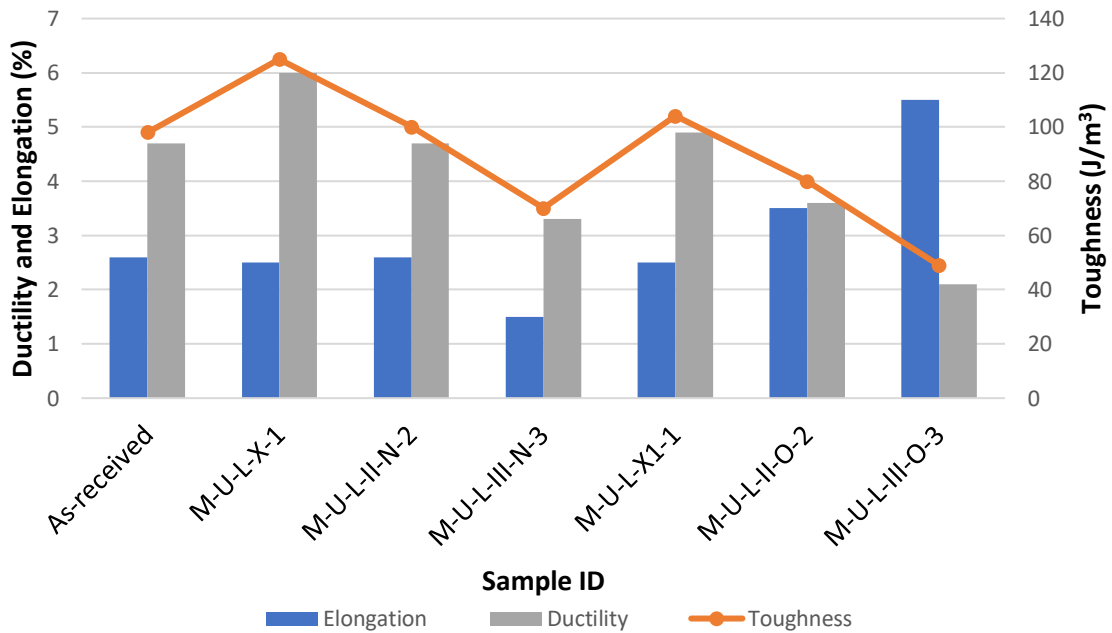
Figure 12 Comparison of ductility properties for tendons with Low level of pre-stress exposed to ICCP-N & ICCP-O
