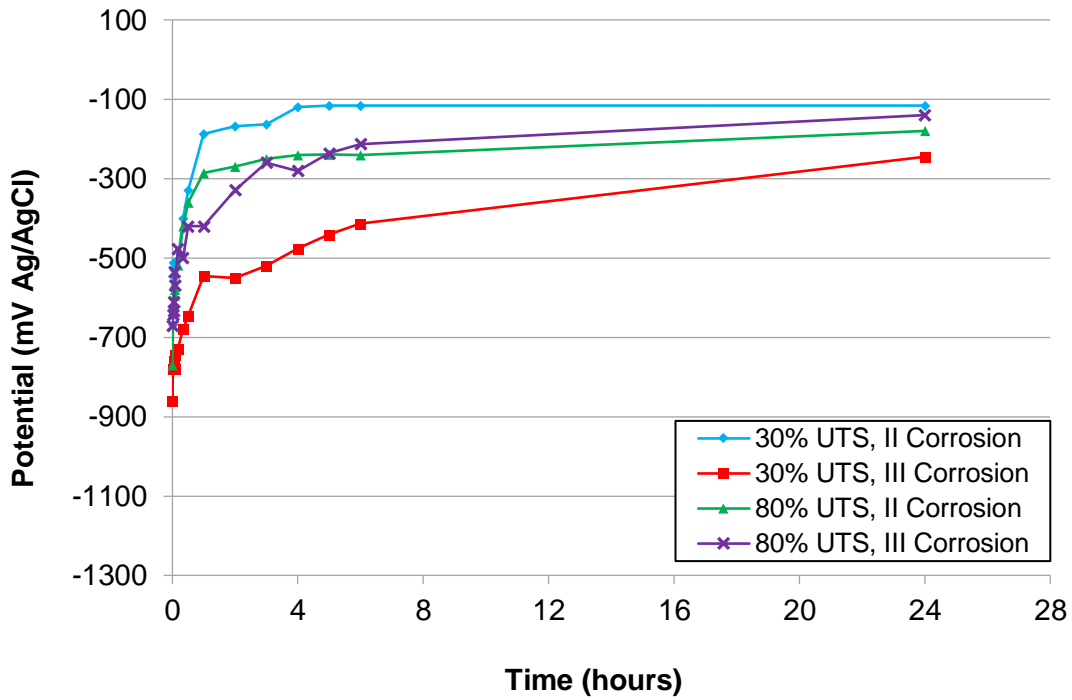
Figure 5 Potential decay of tendons, ICCP-N (Batch 1 & 2)
