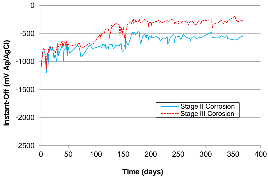
Figure 3 E_{off} for High pre-stressed tendons (Batch 2)
