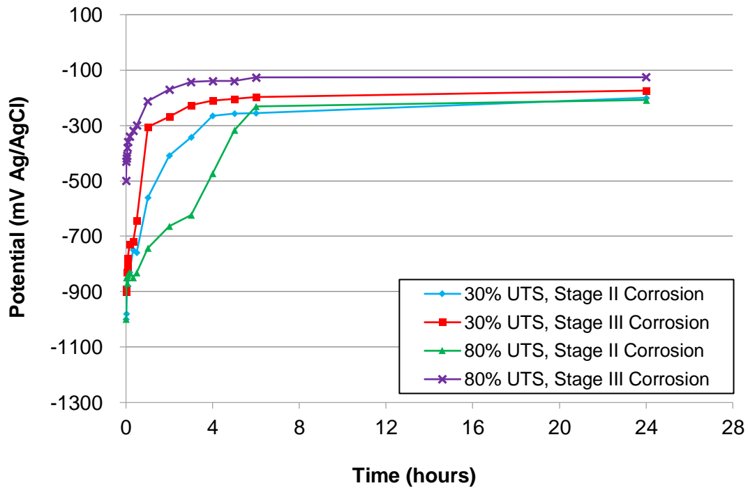
Figure 6 Potential decay of tendons, ICCP-O (Batch 3 & 4)
