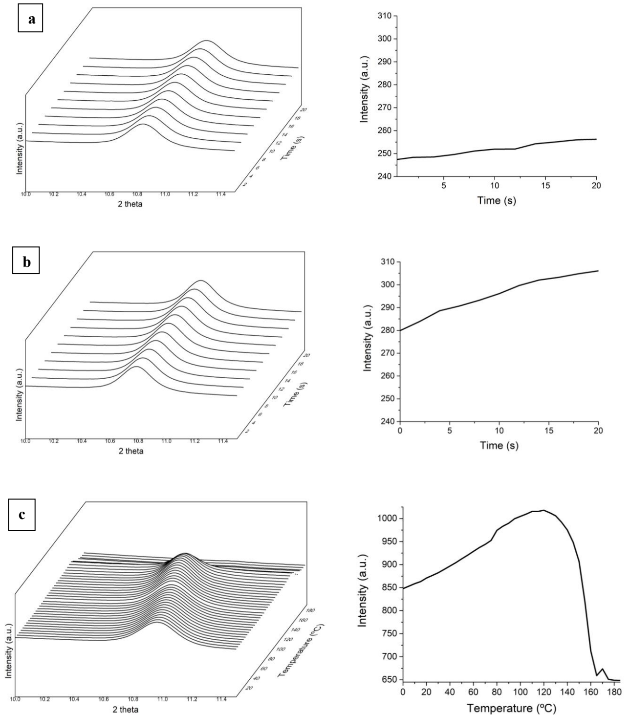
Figure 7. Small angle X-Ray diffraction (SAXS) (left) and wide angle X-Ray diffraction (WAXS) (right) patterns evolution of the electrospun municipal biowaste (MBW) derived poly(3-hydroxybutyrate-co-3-hydroxyvalerate) (PHBV) fibers at: (a) 100 °C for 20 seconds, (b) 130 °C for 20 seconds and (c) during a thermal ramp from 0 °C up to 180 °C at 10 °C/min.
