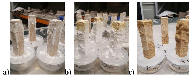
Figure 3. Salt resistance. 2a Anston (type 1) after 120 hours NaCl; 2b Anston (type 1) after 120 hours after 22 days Na 2 SO 4 ; 2c Anston (type 1) after 30 days MgSO 4
