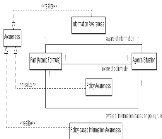
Fig 3 Awareness Association Components in MAAP.
