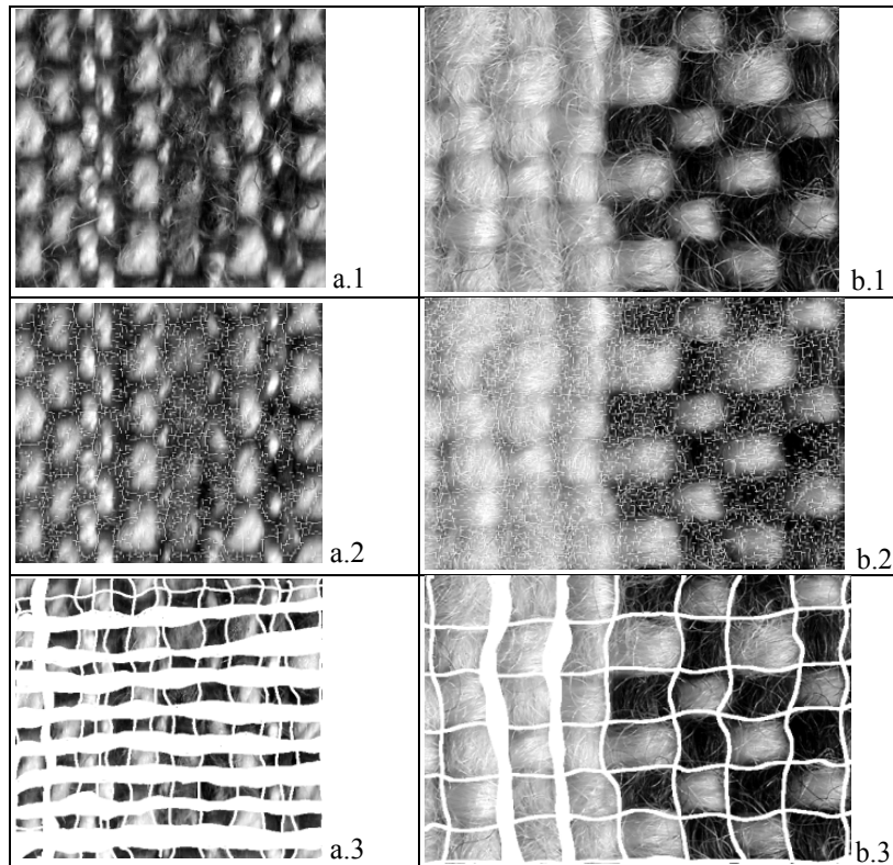
Fig. 2. Crossed-points detection for two samples a and b
