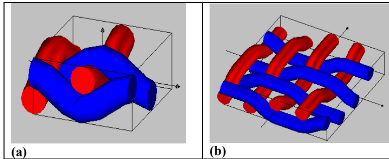
Fig. 5. 3D geometric model for: a) A plain artifact sample b) A twill artifact sample
