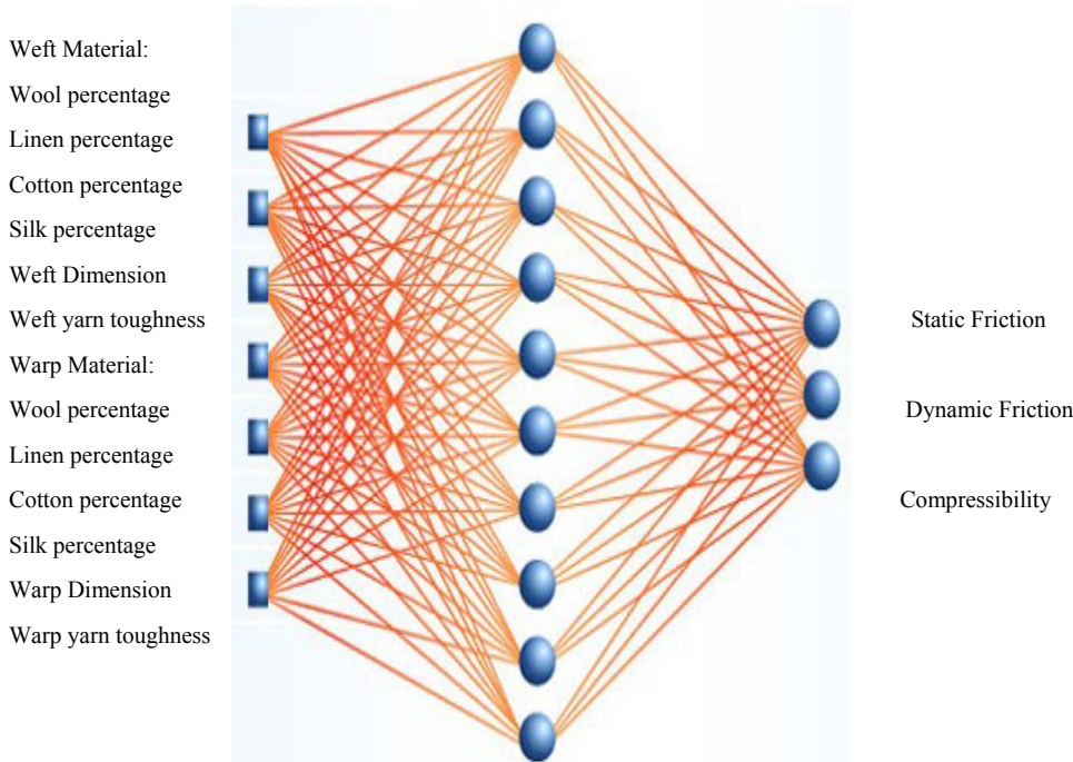
Fig. 7. Neural Network system for textile mechanical & physical properties prediction
