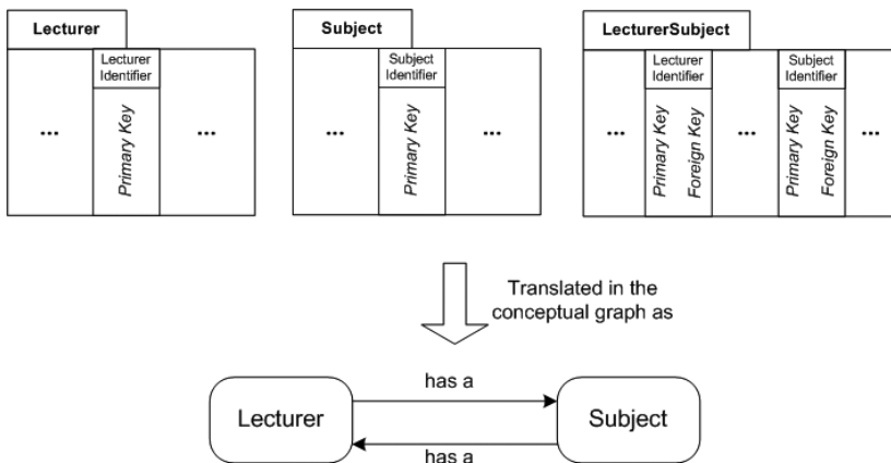
Figure 2: An example of the Mapping Rule 1 (MR1)
