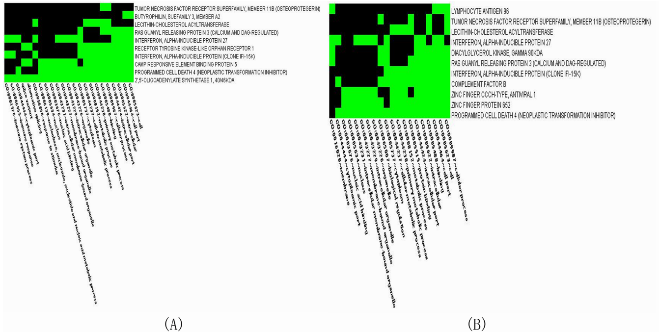
Fig. (2). IFI27 upstream function modules by DAVID in the frontal cortex of HIVE-control patients (A). IFI27 upstream function modules by DAVID in HIVE (B). Green color represents gene-term association positively reported, black color represents gene-term association not reported yet.
