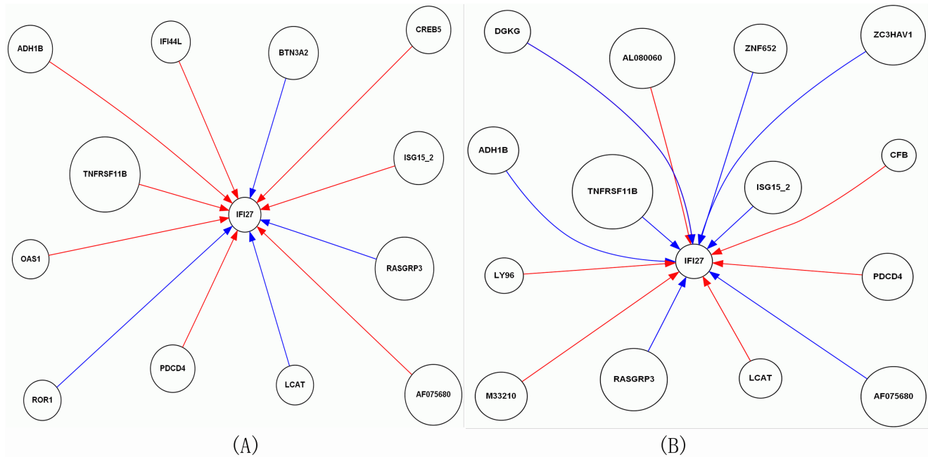
Fig. (1). IFI27 upstream network construction in the frontal cortex of HIVE-control patients by infer (A). IFI27 upstream network construction in HIVE by infer (B). Red color represents activation, blue color represents inhibition.
