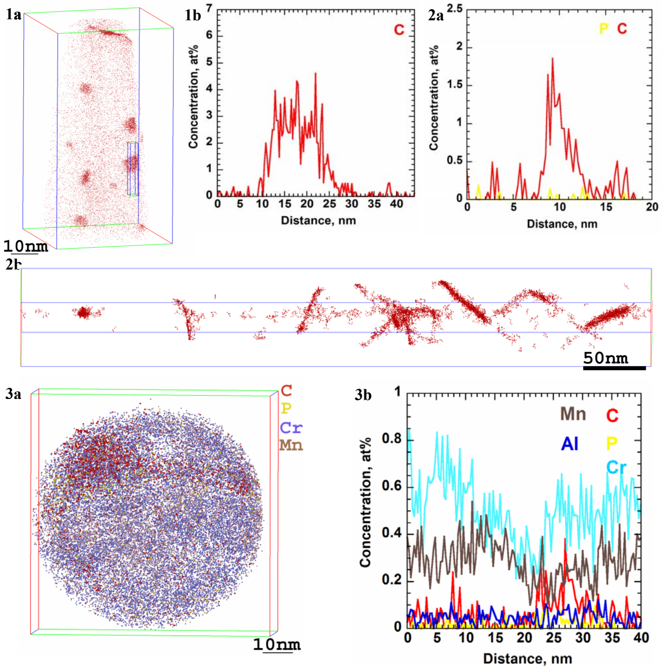
Fig. 1 (a) Atom map showing C clusters in Cr steel and (b) corresponding concentration profile along the blue line of selection box shown in (a).
