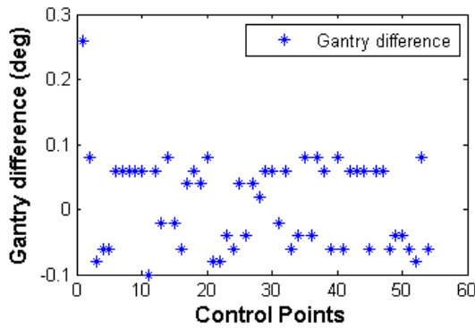
Figure 3: Gantry positional error plot generated by Treat Check for a prostate VMAT plan.
