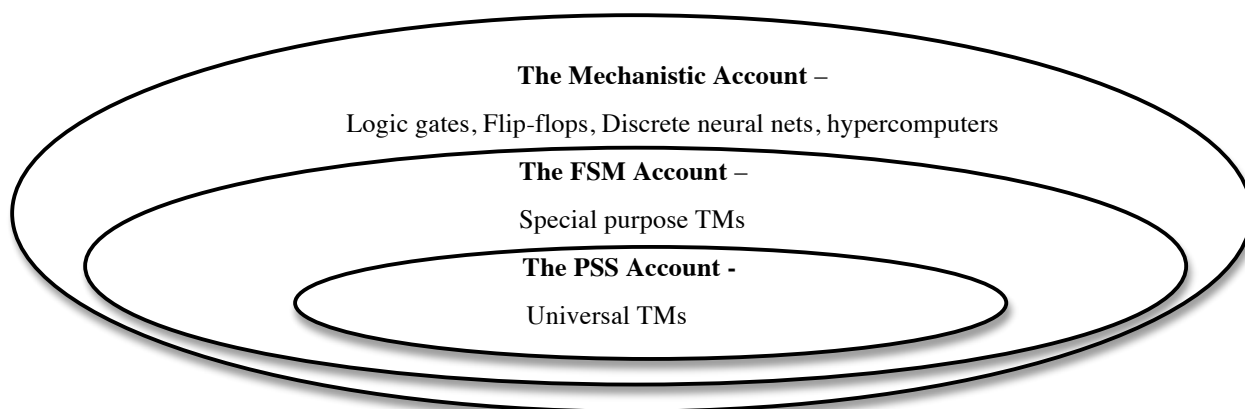
Fig. 1. With the exception of hypercomputers, UTMs are the most powerful and flexible computing systems in the class above (e.g., they can simulate any discrete neural net). Still, UTMs (and physical approximations thereof) do not exhaust all types of digital computing systems. The Mechanistic account is the broadest of the three accounts examined.
