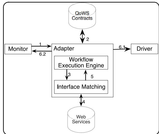
Figure 6 Severe QoWS Adaptation
