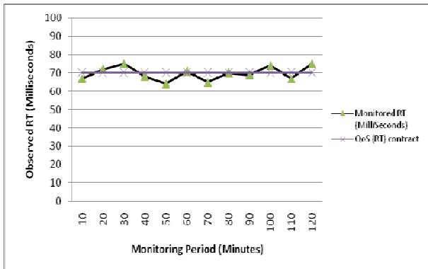
Figure 12. Observed RT after graceful QoS adaptation
