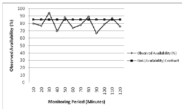
Figure 9. Observed Availability before adaptation
