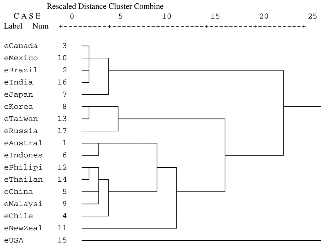
Figure 5 Cluster analysis
