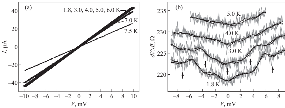
FIG. 2. I - V curves of Nb/Ti-C-Ti/Nb device (G1) at various temperatures from 1.8 to 7.5 K (a). Numerical derivatives, dV/dI ( \Omega ), for the I - V curves measured at different temperatures T , K (thin grey lines). Curves for 3.0, 4.0, and 5.0 K are arbitrarily shifted in vertical direction for clarity. Thick black lines are averaged curves (see text for details) (b).
