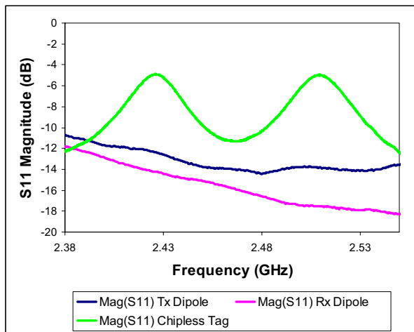
Fig. 25. Measured return loss of the reader dipoles (blue and pink) and the resonance of the multiresonator (black).
