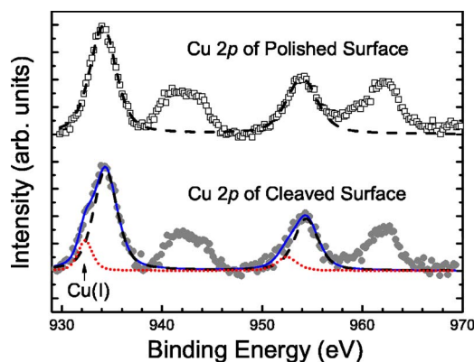
FIG. 3. (Color online) Analysis on \text{Cu } 2p spectra of the cleaved and polished surfaces of \text{CaCu}_3\text{Ti}_4\text{O}_{12} ceramics. Note that the background was subtracted by using Shirley-plus-linear method.
