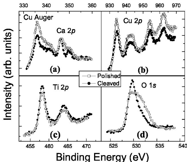
FIG. 2. Core-level spectra of \text{Ca } 2p (a), \text{Cu } 2p (b), \text{Ti } 2p (c), and \text{O } 1s (d) for the cleaved and polished surfaces of \text{CaCu}_3\text{Ti}_4\text{O}_{12} ceramics.
