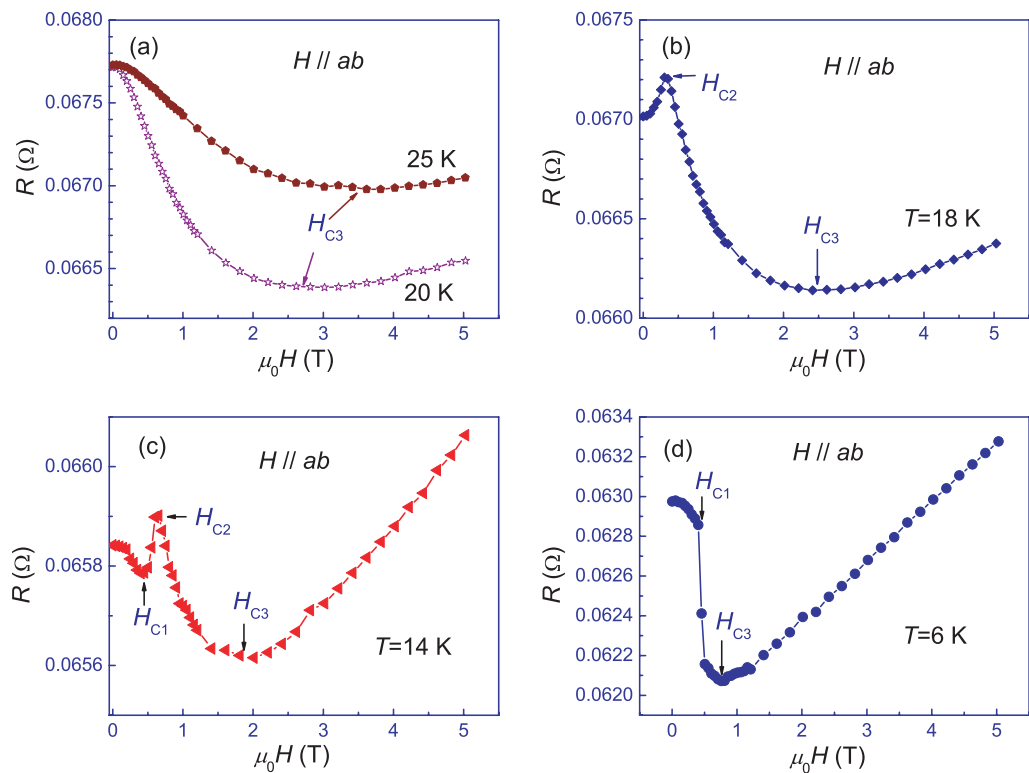
Figure 7. Expanded R_{ab}(H) curves with magnetic field parallel to the ab planes at some representative temperatures for \text{EuFe}_2\text{As}_2 crystals.
