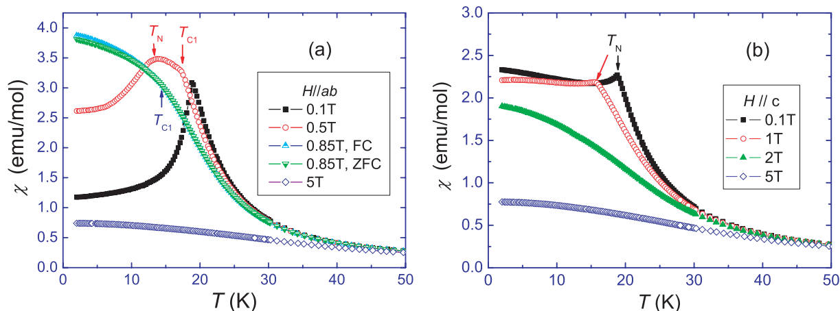
Figure 3. Temperature dependence of magnetic susceptibility of \text{EuFe}_2\text{As}_2 crystals under various magnetic fields. The magnetic field is perpendicular (a) and parallel (b) to the crystallographic c -axis.
