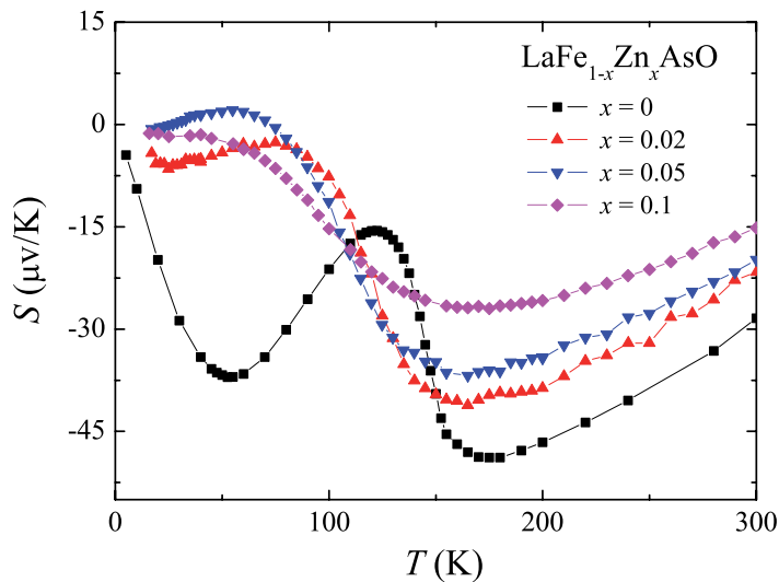
Figure 4. The temperature dependence of thermopower ( S ) for \text{LaFe}_{1-x}\text{Zn}_x\text{AsO} samples.
