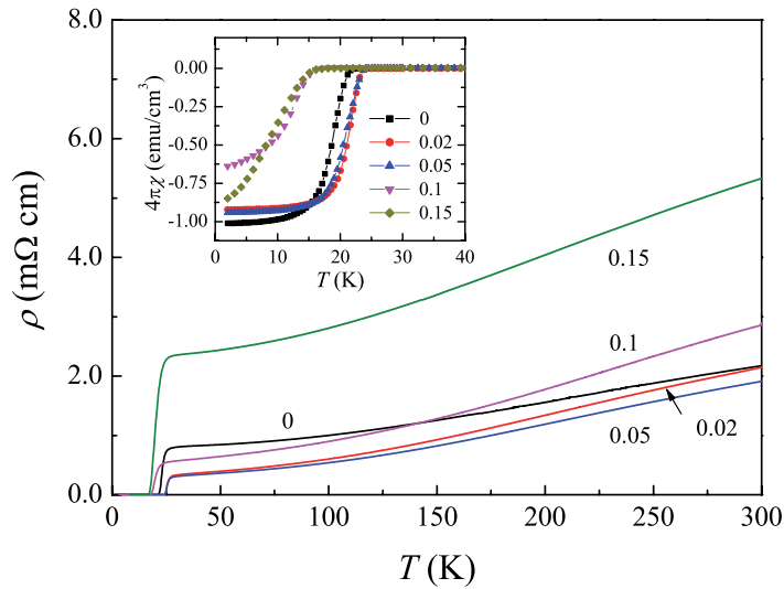
Figure 6. The temperature dependence of resistivity ( \rho ) of \text{LaFe}_{1-x}\text{Zn}_x\text{AsO}_{0.9}\text{F}_{0.1} samples. Inset: the dc magnetic susceptibility ( \chi ) versus temperature measured under magnetic field of 10 Oe.
