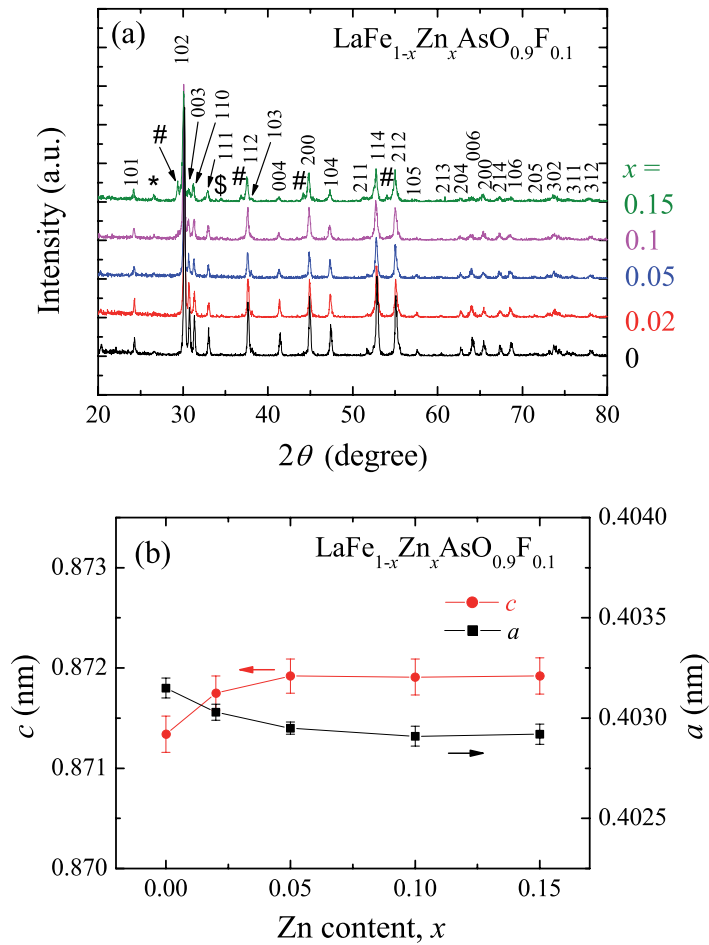
Figure 5. (a) Powder XRD patterns of \text{LaFe}_{1-x}\text{Zn}_x\text{AsO}_{0.9}\text{F}_{0.1} ( x = 0, 0.02, 0.05, 0.1 and 0.15 ) samples. The symbols #, \star and \$ denote the impurity phases \text{LaZnAsO} , \text{La}_2\text{O}_3 and \text{FeAs} , respectively. (b) Lattice parameters as a function of Zn content.
