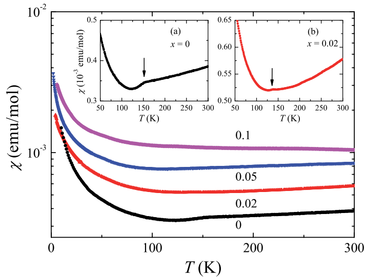
Figure 3. The temperature dependence of magnetic susceptibility ( \chi ) of \text{LaFe}_{1-x}\text{Zn}_x\text{AsO} samples. The insets show the enlarged plots for x = 0 and 0.02 . The arrows indicate the anomaly in susceptibility related to structural and/or magnetic transitions.
