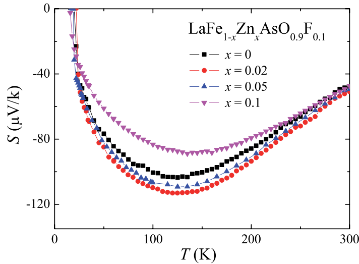
Figure 7. The temperature dependence of thermopower ( S ) for \text{LaFe}_{1-x}\text{Zn}_x\text{AsO}_{0.9}\text{F}_{0.1} samples.
