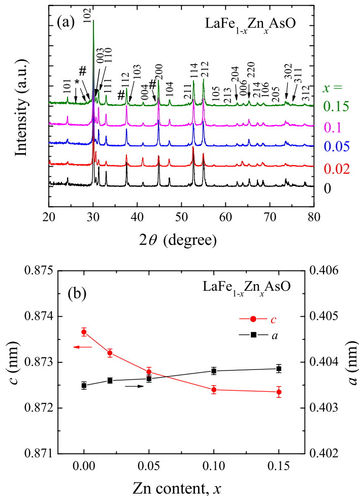
Figure 1. (a) Powder XRD patterns of \text{LaFe}_{1-x}\text{Zn}_x\text{AsO} ( x = 0, 0.02, 0.05, 0.1 and 0.15 ) samples. The symbols \# and \star denote the impurity phases \text{LaZnAsO} and \text{La}_2\text{O}_3 , respectively. (b) Variations of lattice parameters as a function of Zn content.
