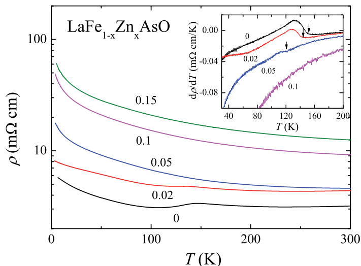
Figure 2. The temperature dependence of resistivity ( \rho ) for \text{LaFe}_{1-x}\text{Zn}_x\text{AsO} samples. The inset shows the derivative of resistivity versus temperature. The arrows indicate the anomaly in resistivity, which could be associated with structural and/or magnetic transitions.
