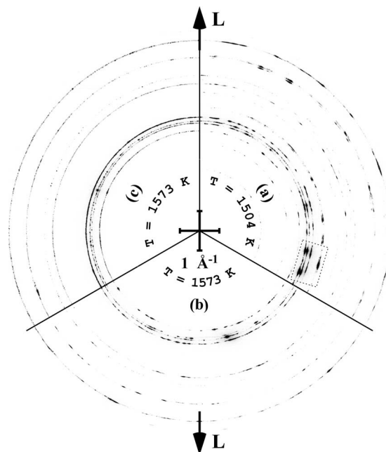
FIG. 1. Representative parts of the acquired diffraction rings compiled in three sectors: (a) below the alpha transus temperature T_\alpha , showing \alpha -, \beta -, and \gamma -phases in coexistence; (b) above T_\alpha , where \gamma disappeared before plastic deformation and (c) above T_\alpha during plastic deformation. Reflections in the indicated box in (a) reveal orientation correlations of all three phases. The common ring center is marked with a crossed scale bar of 1 \text{ \AA}^{-1} and the longitudinal load direction L is indicated. Reflections are indexed in Fig. 2.
