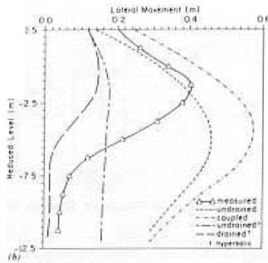
FIG. 14. Variation at Location of inclinometer, I3: (a) Lateral Displacement Response at 4.5 m Depth; (b) Lateral Displacement Profile at Failure
