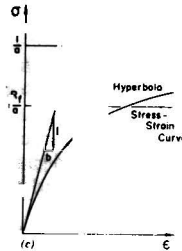
FIG. 10. Parameters Required for Hyperbolic Stress-Strain Model (Ozawa and Duncan 1973)
