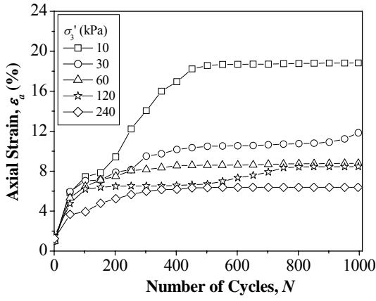
Figure 2. Variation of \epsilon_a with N at different \sigma'_3
