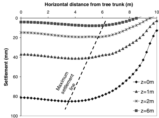
Figure 8. Ground settlement at various depths
