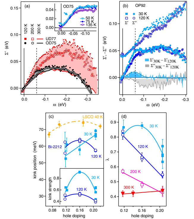
FIG. 2 (color online). (a), (b) Self-energy functions derived from experimental data for an overdoped, underdoped, and optimally doped Bi-2212 samples; the inset in (a) shows the data for OD75 taken \approx 0.15 \text{ \AA}^{-1} away from the node to monitor the gap opening; on (b) the solid curve shows a fit of \Sigma'(30 \text{ K}) - \Sigma'(120 \text{ K}) to a Gaussian. (c), (d) The evolution of the kink parameters with hole concentration and temperature; different points correspond to different samples; the error bars are derived from a number of measurements of each sample.
