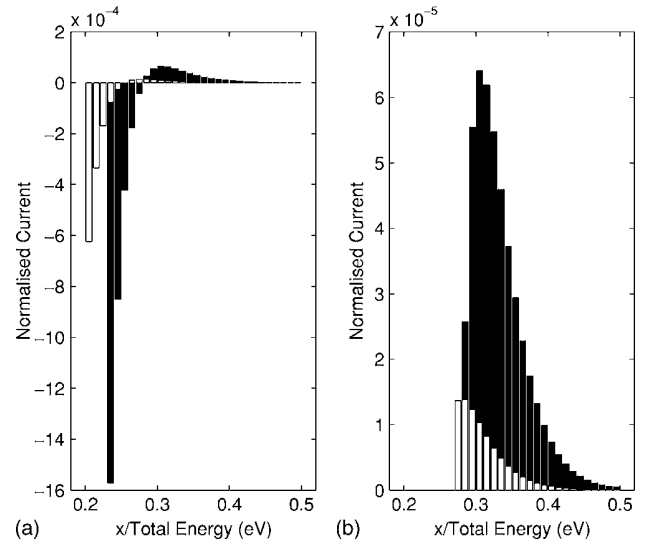
FIG. 4. The normalized electron energy spectrum for net current from the hot to cold reservoir. The filter width is 0.3 eV and is positioned to achieve maximum efficiency/COP in each system for (a) refrigeration and (b) power generation in k_r (black) and k_x (white) systems. T_C=270 K, T_H=300 K, and \mu_C=0.1 eV, \mu_H=0.08 eV.
